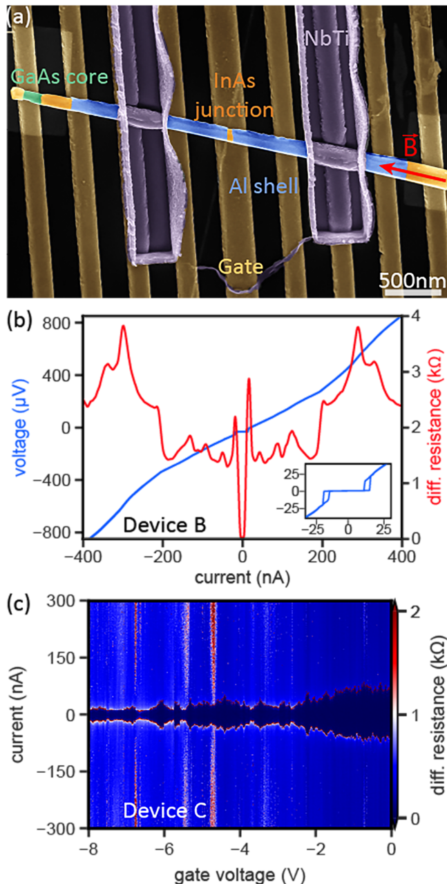
Fig. 3 | Supercurrent and Andreev transport in GaAs/InAs/Al Josephson junctions. a False-colored scanning electron micrograph of an exemplary GaAs/InAs/Al core/shell/halshell nanowire Josephson junctions with an approx. 140 nm long channel. b Current-voltage characteristics (blue) and differential resistance (red) as a function of bias current of device B at T = 14 mK and a gate voltage of V_g = 0 V. The inset shows detail around the supercurrent branch of the I - V trace, revealing an underdamped behavior. c Differential resistance as a function gate voltage and bias current for device C at T = 14 mK.
