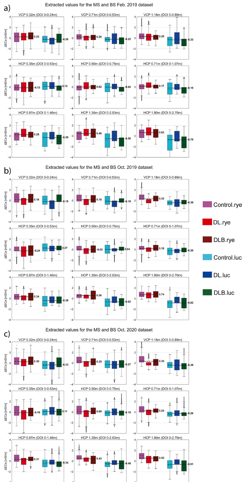
Fig. 6. Boxplots of \Delta ECa values extracted from the rectangular sampling areas for all coil configurations for the mean subtraction (MS) and background subtraction (BS) February 2019, October 2019, and October 2020 datasets. The boxplots illustrate the variability of soil ECa across the six management treatments (Control.rye, DL.rye, DLB.rye, Control.luc, DL.luc, DLB.luc). In the graphs, moving from left to right, increasing subsoil manipulations are observed (rye: Ryegrass cover crops; luc: Lucerne cover crops; Control: reference-control; DL: deep tillage; DLB: deep tillage with biowaste).
