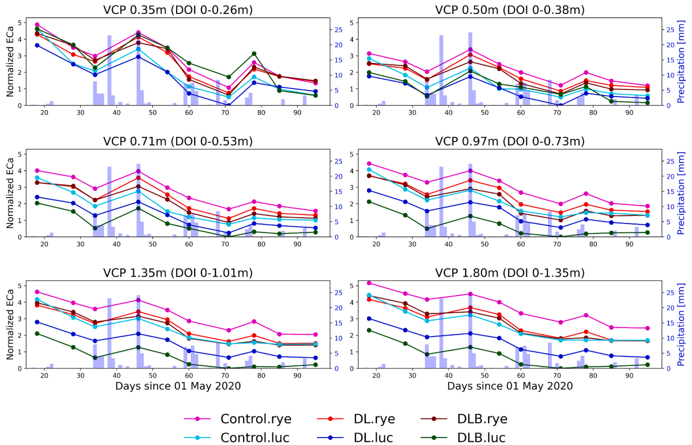
Fig. 7. Normalized mean ECa values derived from point-scale measurements collected in summer 2020 and grouped by soil treatment, as a function of the spring barley growth period for different VCP configurations (0.35, 0.50, 0.71, 0.97, 1.35, 1.80 m). Local measured precipitation (mm) is also reported in the graphs as blue histograms.
