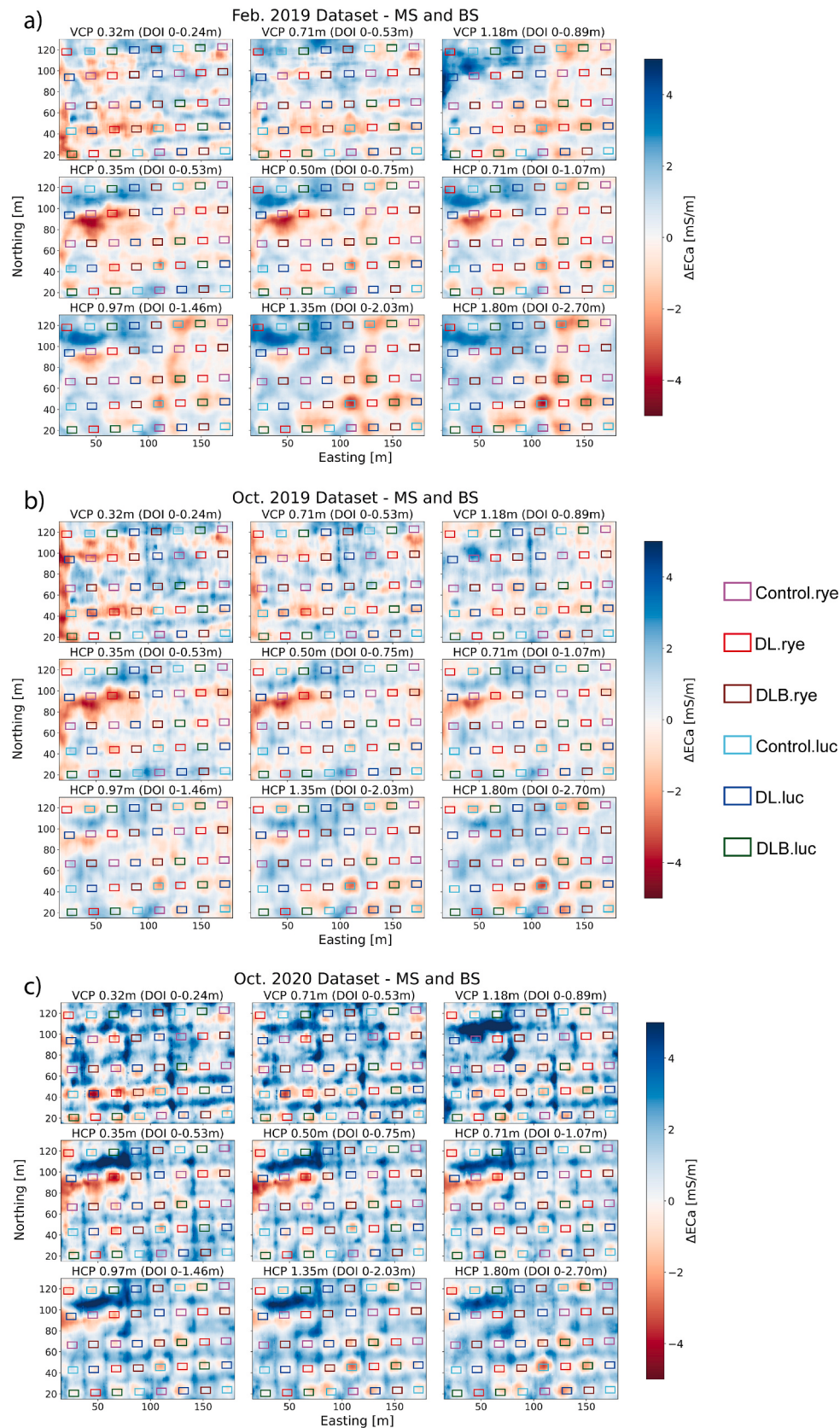
Fig. 5. ECa maps for the February 2019, October 2019, and October 2020 datasets obtained through the data-processing workflow developed in this study. For each coil configuration, all datasets were normalized by subtracting the mean subtraction (MS) calculated within the shown central rectangular areas. Subsequently, the mean subtracted August 2016 (background) dataset, was subtracted from the three datasets.
