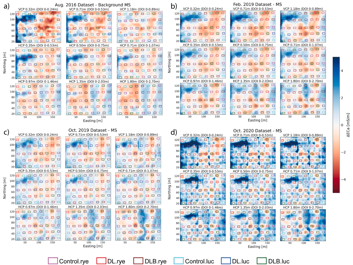
Fig. 4. ECa maps for the August 2016, February 2019, October 2019, and October 2020 datasets normalized by subtracting the mean subtraction (MS) calculated within the centred internal window, centred on the different treatment plots.
