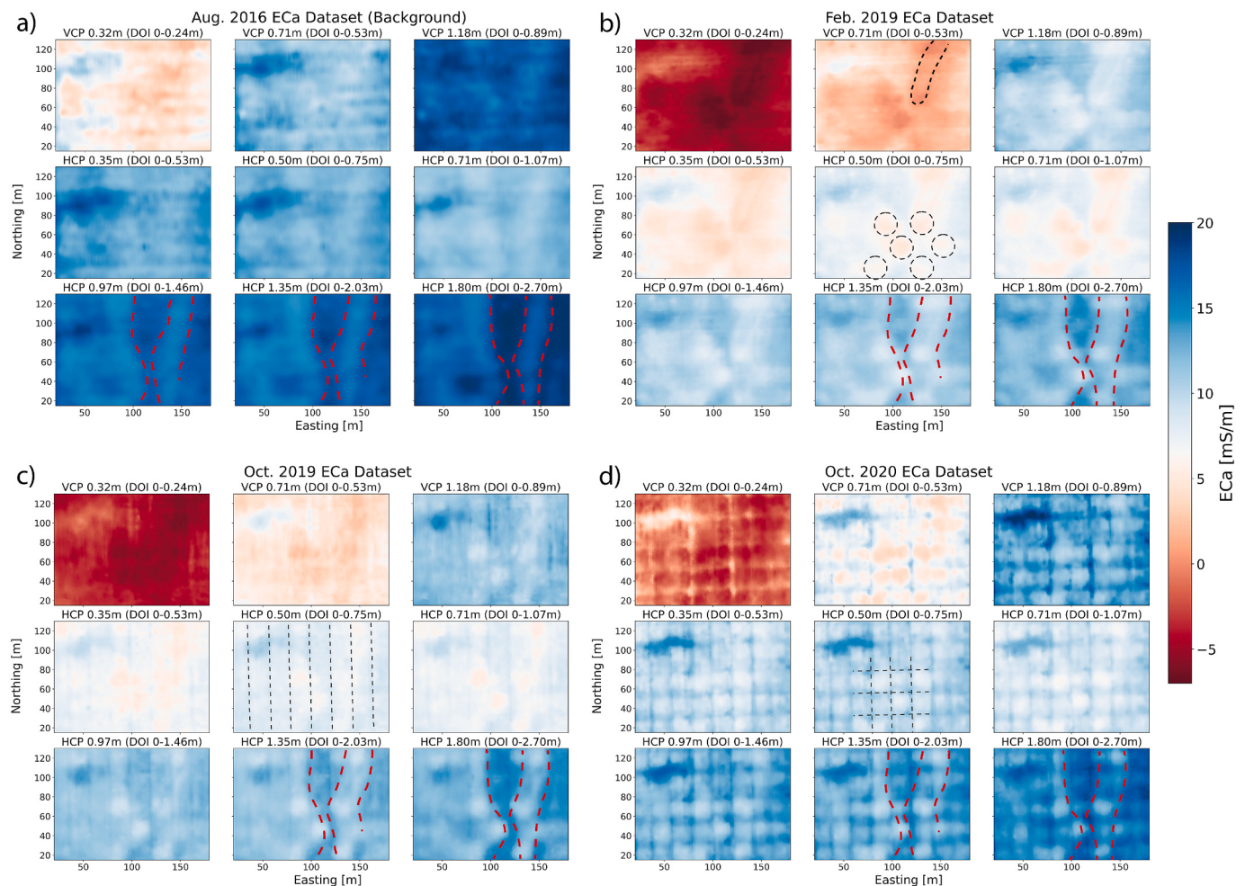
Fig. 3. Filtered and interpolated ECa maps for each field-scale acquisition from August 2016 to October 2020 for the three VCP configurations (0.32, 0.71, and 1.18 m) acquired with the CMD Mini-Explorer, and for the six HCP configurations (0.35, 0.50, 0.71, 0.97, 1.35, and 1.80 m) acquired with the CMD Mini-Explorer Special Edition. Dashed annotations highlight the principal spatial features discussed in the text, including persistent background conductive stripes (red), localized conductivity anomalies (black), and linear patterns associated with the experimental layout and traffic lanes (black).
