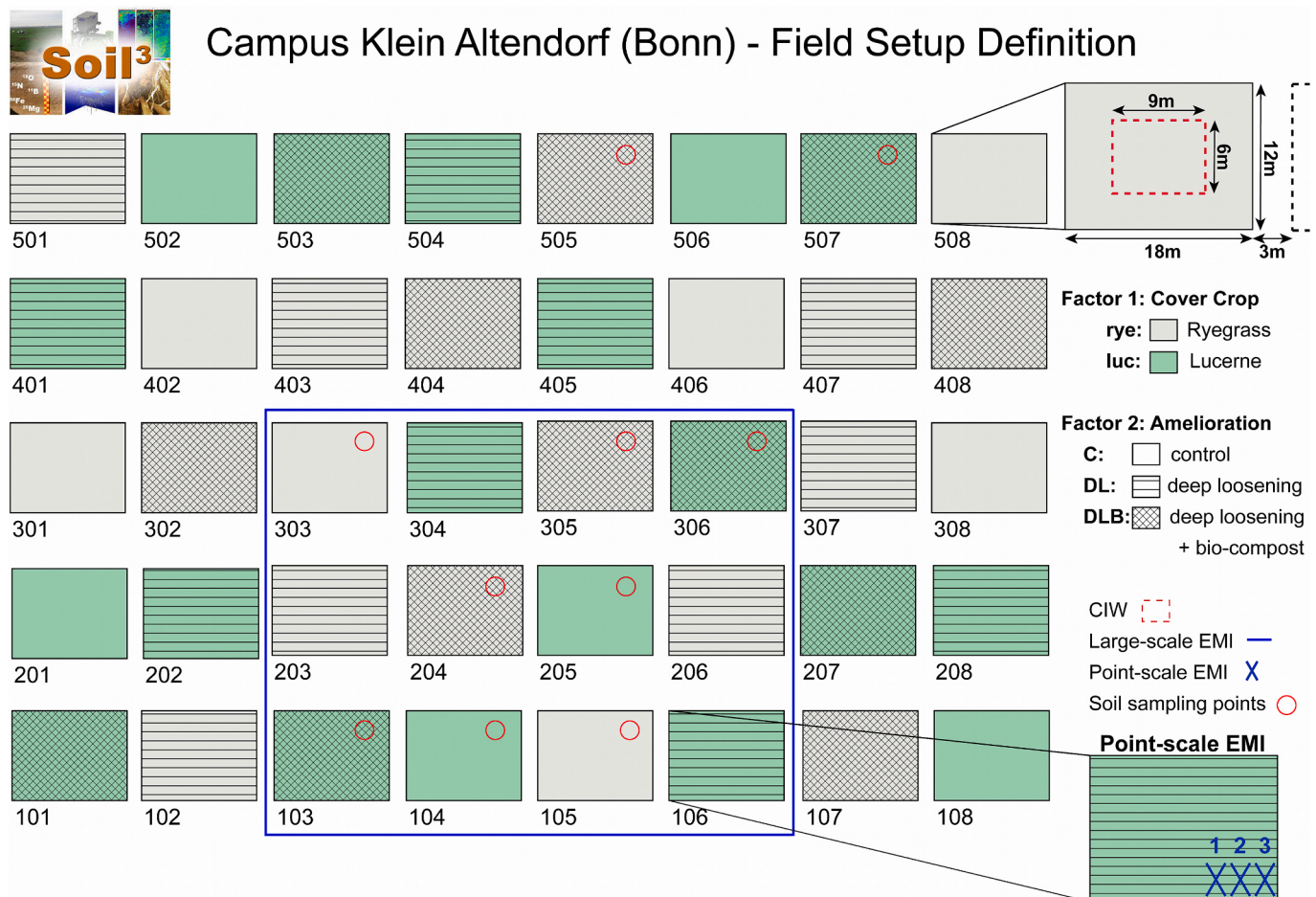
Fig. 1. Schematic representation of the agricultural site studied between 2016 and 2020 as part of the Soil 3 project at the experimental station of the University of Bonn, Campus Klein-Altendorf, Rheinbach, Germany ( 50^{\circ}38'5.71''\text{N} , 6^{\circ}58'37.24''\text{E} ), showing the organization and distribution of cover crops and amelioration practices applied on the site. The blue rectangle identifies the area where the point-scale EMI measurements were carried out. CIW: centred internal window.
