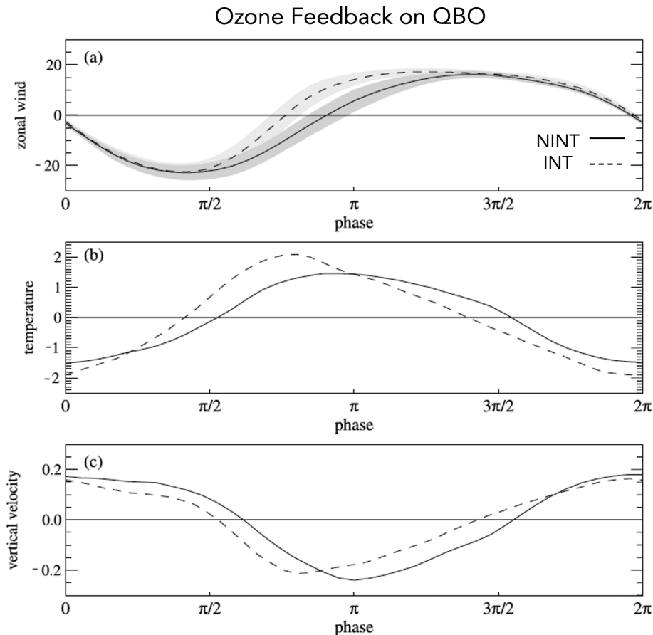
Figure 1. Comparisons of the tropical zonal mean zonal wind ( \text{m s}^{-1} ) (a) and anomalies in temperature (K) (b) and vertical residual velocity ( \text{mm s}^{-1} ) (c) between simulations using specified (NINT, solid line) versus coupled (INT, dashed line) ozone. Fields are evaluated at the equator and at 21.5 hPa and plotted as a function of QBO phase. The data shown is from the model simulations performed using a version of the Met Office Unified Model, as reported in Butchart et al. (2003).
