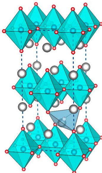
Figure 1. Schematic representation of the \text{Pr}_2\text{NiO}_{4.25} structure (blue: Ni, red: O, gray: Pr) in the average Fmmm cell containing the interstitial oxygen. \text{O}_{\text{int}} atom located in the \text{Pr}_2\text{O}_2 rock salt layer with average occupation of \frac{1}{8} and it is tetrahedrally coordinated by the apical oxygen atoms as well as Pr atoms (blue polyhedron).
