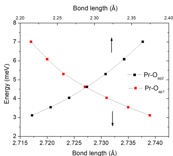
Figure 4. Trend of first CEF level energy obtained through point charge model calculations by varying the atomic positions of O_{\text{ap}} . Red squares are connected to the \text{Pr-O}_{\text{ap1}} bond length, black squares to the \text{Pr-O}_{\text{ap2}} bond length as defined in Figure 2.
