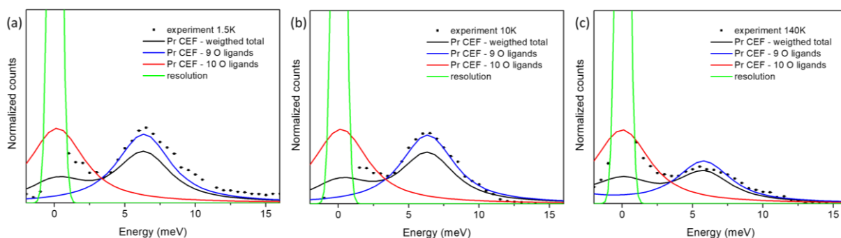
Figure 3. (a) INS spectra of \text{Pr}_2\text{NiO}_{4.25} measured at the IN20 spectrometer at 1.5 K, with the calculated CEF excitations for the LT model. (b) Same as (a) but at 10 K. (c) INS spectra of \text{Pr}_2\text{NiO}_{4.25} measured at the IN20 spectrometer at 140 K, along with the calculated CEF excitations for the HT model. For all plots, black scatter are experimental data, green line is the instrument resolution, blue line is the CEF from Pr ions with 9 ligands, red line is CEF from Pr ions with 10 ligands, black line is the weighted sum.
