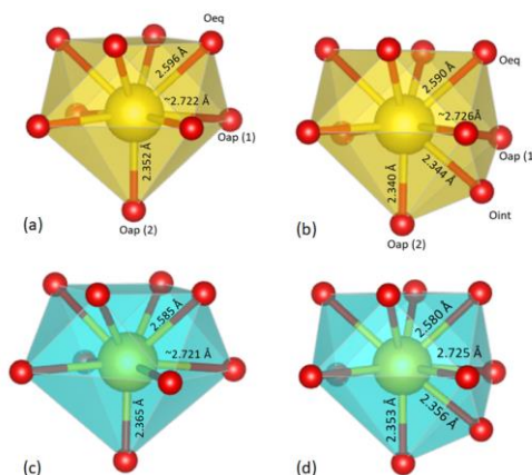
Figure 2. (a) CEF environment of \text{Pr}^{3+} ion HT structural model with twofold rotational z axis (b) CEF environment with an extra \text{O}_{\text{int}} in the HT structure. (c) CEF environment of \text{Pr}^{3+} ion LT structural model with twofold rotational z axis (d) CEF environment with an extra \text{O}_{\text{int}} in the LT structure.
