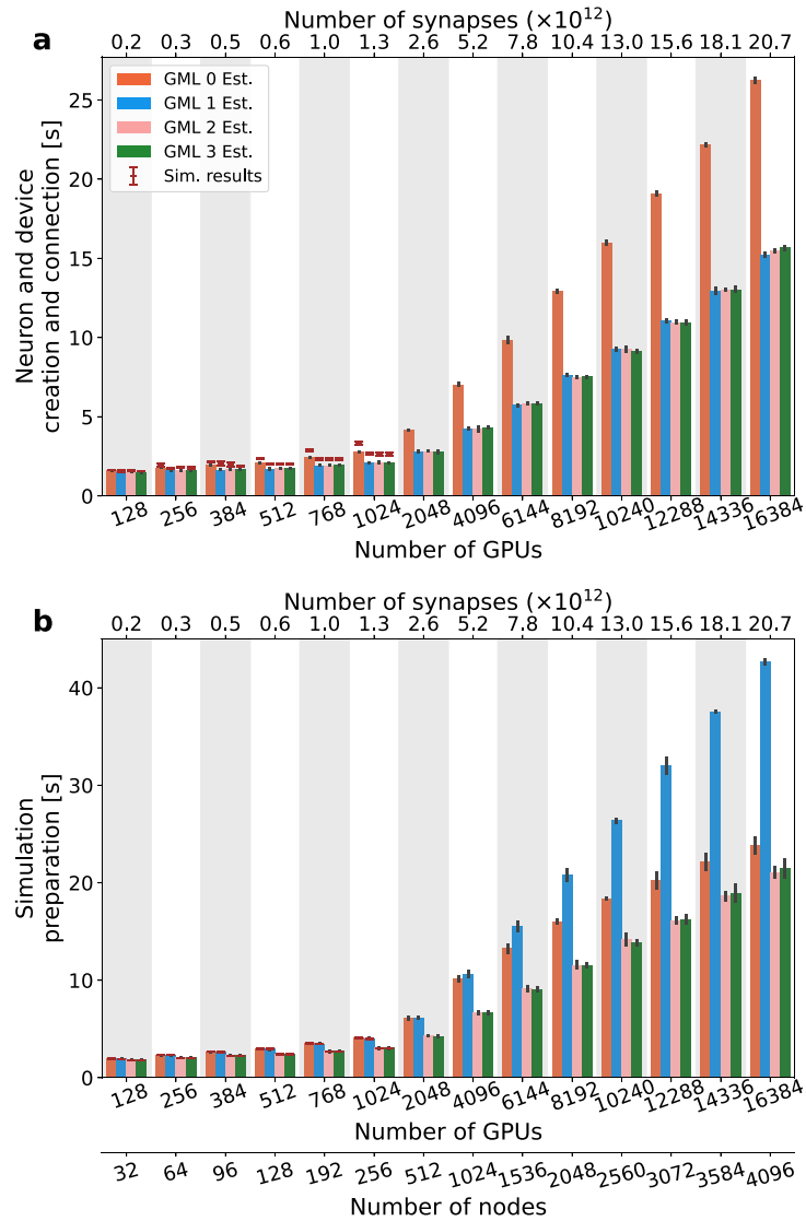
Figure 10. Network construction time divided into neuron creation and connection (a) and simulation preparation (b) times of the scalable balanced network model simulated at scale 10 evaluated across all MPI processes as a function of the number of cluster nodes for the three GPU memory levels. The bars represent an estimation using four MPI processes on a single node. The horizontal line markers show the time averaged across the MPI processes using the GPU memory levels. Errors for bars and horizontal line markers represent their standard deviation, with most of the values showing little variability.
