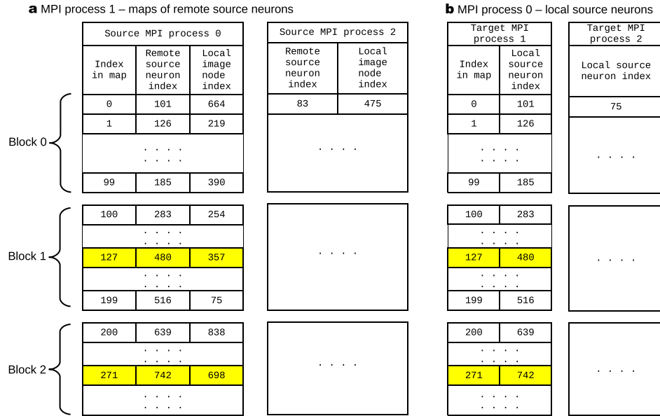
Figure 14. (a) organization of the maps ( R_{\tau,\sigma,i}, L_{\tau,\sigma,i} ), which associate remote source neurons to local image neuron indexes, in the GPU memory of the target MPI process, which has rank \tau = 1 in this example. The left column represents the position in the map, i , while the other two columns represent the remote source neuron index, R_{\tau,\sigma,i} and the local index of its image neuron in the target MPI process, L_{\tau,\sigma,i} . (b) organization of the sequence S_{\sigma,\tau,i} , which represent the local source neuron index, in the GPU memory of the source MPI process, which has rank \sigma = 0 in this example. The left column represents the position in the sequence, i , while the other column represent the local source neuron index, S_{\sigma,\tau,i} .
