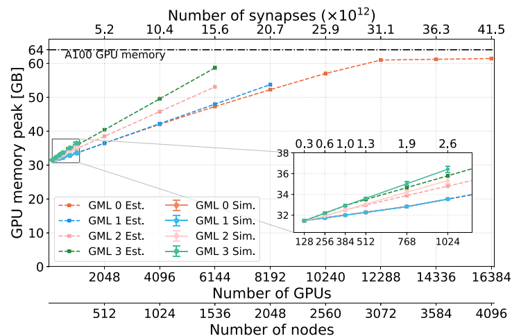
Figure 5. Peak memory usage per GPU for the scalable balanced network model simulation as a function of the number of cluster nodes for the four GPU memory levels. The upper horizontal axis shows the total number of synapses of the model, indicating the increasing network size. Square markers and dashed lines represent the estimation of the memory peak obtained using four MPI processes on a single node. Dot markers and continuous lines represent simulated configurations over five simulations using different random seeds. Error bars represent standard deviations. On the bottom right of the figure, an inset of the measured data is shown to facilitate comparison with the estimated values. Dash-dotted horizontal line represents the memory limit of one NVIDIA A100 GPU. For these configurations, the first two levels of GPU memory show compatible results, and the points overlap.
