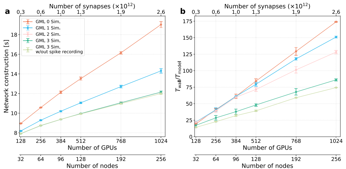
Figure 4. Network construction (a) and state propagation (b) times of the scalable balanced network model for the four GPU memory levels as a function of the number of cluster nodes (four GPUs per node). State propagation is measured as the real-time factor. The GPU memory level 3 was also reported when spike recording was disabled. GPU memory levels 2 and 3 in the network construction overlap.
