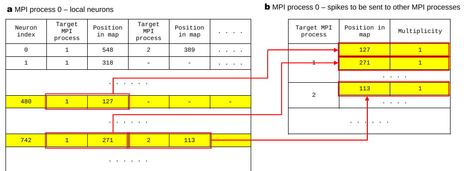
Figure 15. (a) organization of the sequences T_{\sigma,s,j} , which represent the ranks of the target MPI processes in which each node has an image, and P_{\sigma,s,j} which are the corresponding positions of the neuron in the maps that associate it to its image neurons in the target processes. (b) creation of the packets to be sent to target MPI processes using point-to-point MPI messages. In this example we assume that in a certain time step nodes 480 and 742 of the MPI process 0 emit a spike. We can observe that node 480 has an image in the target process 1, and that the corresponding position in the maps is 127, while node 742 has images in the MPI processes 1 and 2, and the corresponding positions are 271 and 113, respectively. These positions are appended to the packets created for the respective target MPI processes, which will be sent via point-to-point communication.
