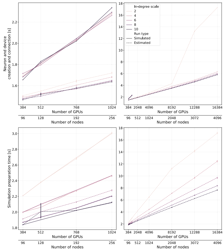
Figure 12. Neuron and device connection and creation and simulation preparation times of the scalable balanced network model for different values of in-degree_scale as a function of the number of cluster nodes (four GPUs per node). Panels on the left represent the results in the range of compute nodes for which simulations are executed, whereas right panels extend to the range in which the performance is evaluated with the estimation method. Lines represent simulated results, whereas dotted lines represent estimated results. Vertical bars indicate the standard deviation.
