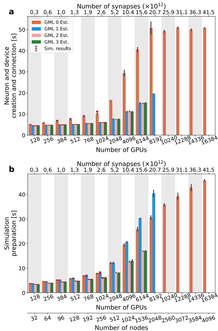
Figure 6. Network construction time divided into neuron creation and connection—panel (a) contribution of the neuron and device creation and the local and remote connection generation subtasks—and simulation preparation—panel (b) organization of data structures for spike delivery subtask—times of the scalable balanced network model evaluated across all MPI processes as a function of the number of cluster nodes for the three GPU memory levels. The bars represent an estimation using four MPI processes on a single node. The horizontal line markers show the time averaged across the MPI processes of five simulations with different seeds using the GPU memory levels. Errors for bars and horizontal line markers represent their standard deviation, with most of the values showing little variability.
