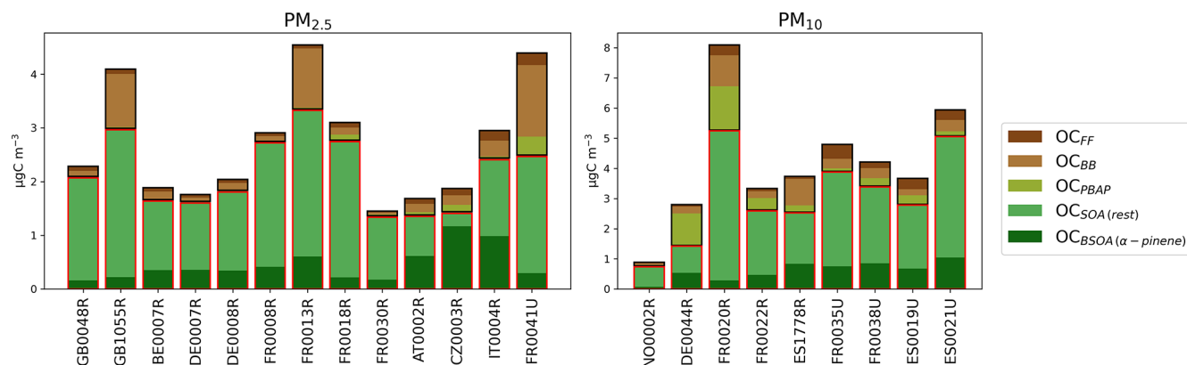
Figure 12. OC apportioned into categories with \text{PM}_{2.5} (left) and \text{PM}_{10} (right) size fractions. Secondary OCs are indicated with a red border and primary OCs with a black border.
