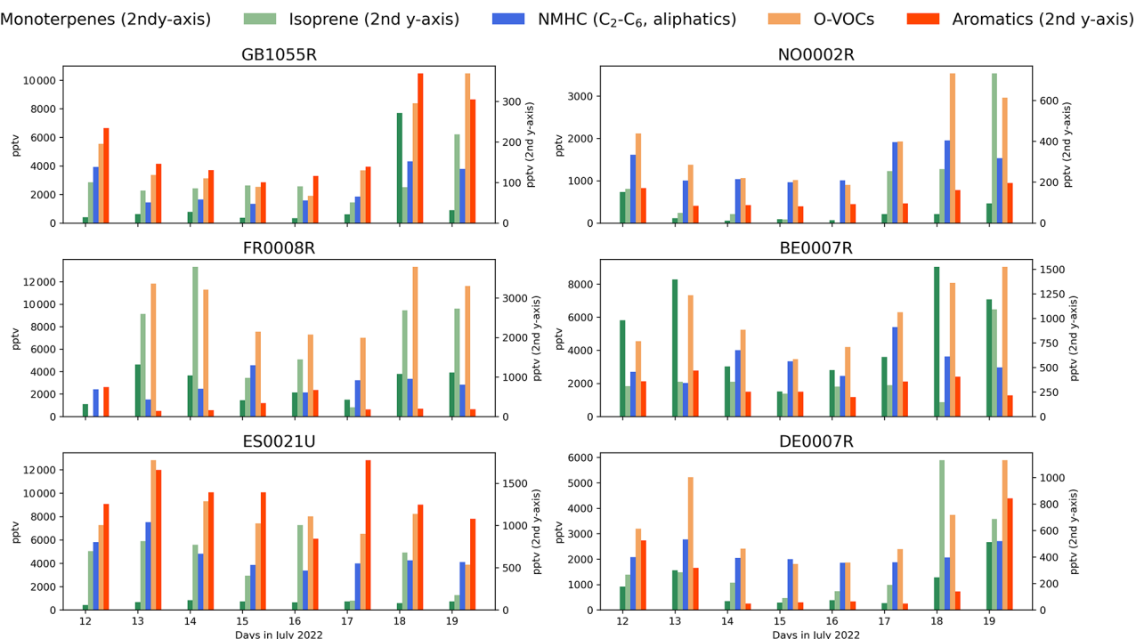
Figure 7. Temporal variations of selected VOCs and VOC groups at 6 sites across Europe on 12–19 July.
