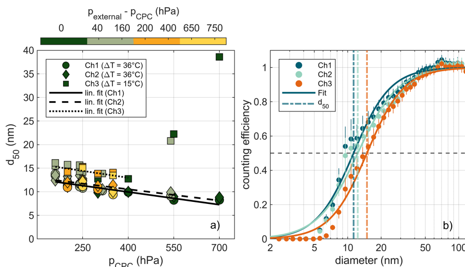
Figure 8. (a) FZJ measurements for all mc-CPC channels plotted as cutoff diameters dependent on p_{CPC} , color coded by \Delta p = p_{external} - p_{CPC} ; and (b) normalized counting efficiencies with corresponding cutoff diameters measured and averaged at p_{CPC} = 250 hPa and p_{external} = 300 and 400 hPa. The data points represent the mean values of two measurement steps for p_{external} = 300 and 400 hPa in each case at two different days. The error bars are the standard deviation of these four combined measurements.
