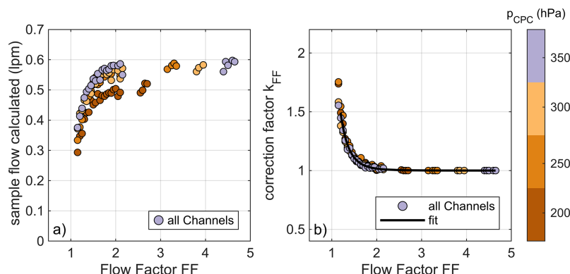
Figure C1. (a) Sample flow of all three mc-CPC channels combined measured by a TSI flowmeter against the Flow Factor FF, (b) correction factor k_{FF} ( = \text{flow}_{\text{max}} / \text{flow} ) derived from the sample flow, color coded by the internal pressure. The measurements were done at GUF. The data points represent averaged data.
