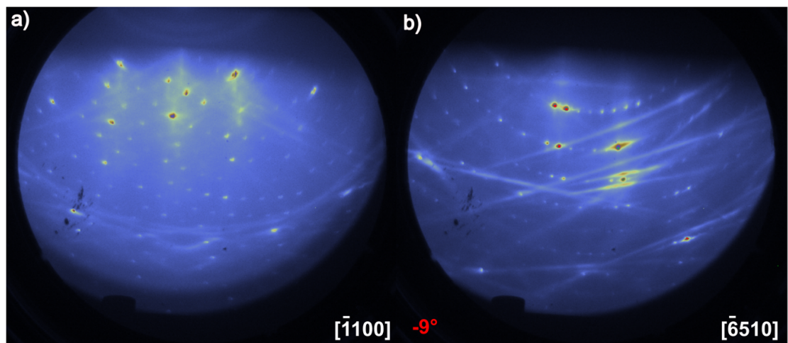
Figure A1. RHEED images of the reconstructed sapphire surface produced after being heated to 1700^\circ\text{C} for 200 s in UHV conditions. Prior to imaging, these substrates were stored in air for six months. The sample was baked in a UHV atmosphere at 400^\circ\text{C} for 30 min prior to imaging in order to remove any volatile absorbates resulting from extended storage in air. Images were taken along the [1100] direction, shown in (a) and the [6510] direction, taken by rotating the sample by 9^\circ anti-clockwise (while viewing the substrate from the top). This image is shown in (b) Both of these images are consistent with prior literature of the double-step ( \sqrt{31} \times \sqrt{31} ) R \pm 9^\circ surface reconstruction [20].
