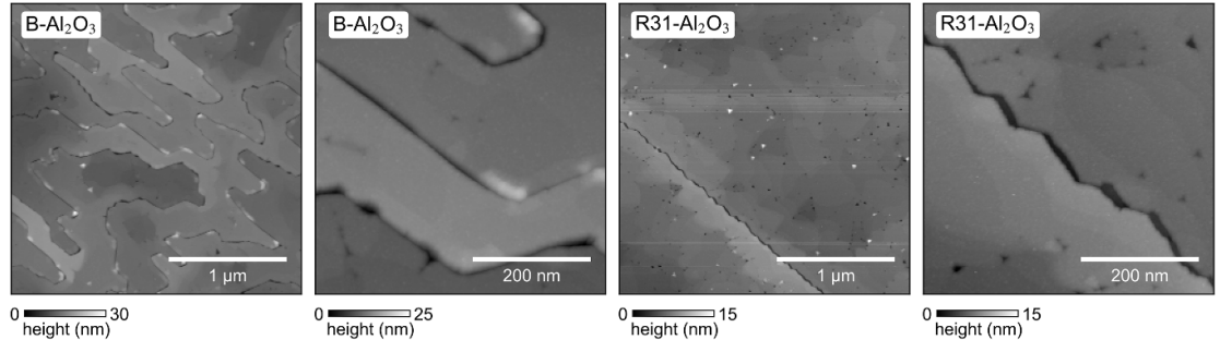
Figure D4. STM topographs of d = 106 nm thick TiN films grown on chemically cleaned (B- \text{Al}_2\text{O}_3 ) and thermally reconstructed (R31- \text{Al}_2\text{O}_3 ) sapphire substrates (current setpoint: 30 pA, bias voltage: 800 mV).
