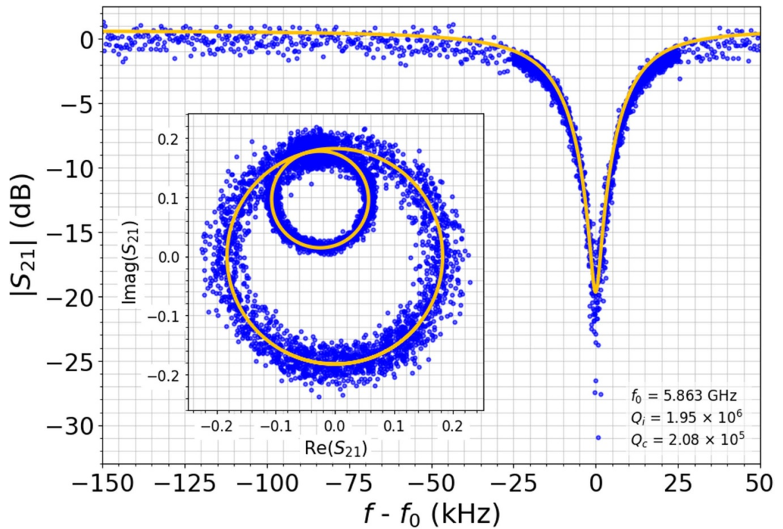
Figure E7. S_{21} as a function of frequency, f for a TiN resonator on B- \text{Al}_2\text{O}_3 with a resonant frequency, f_0 = 5.863 GHz. All data was taken at T \sim 25 mK and measured at a microwave power of -150 dBm corresponding to \langle n \rangle \sim 2.52 .
