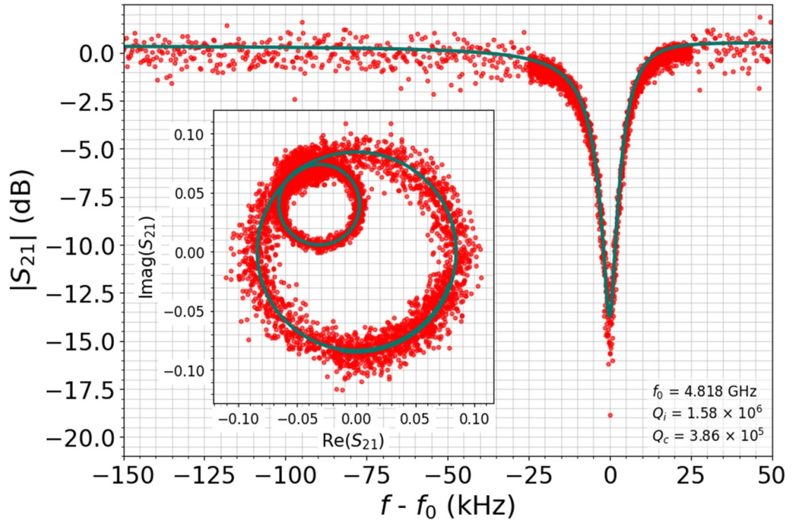
Figure E6. S_{21} as a function of frequency, f for a TiN resonator on R31- \text{Al}_2\text{O}_3 with a resonant frequency, f_0 = 4.818 GHz. All data was taken at T \sim 20 mK and measured at a microwave power of -155 dBm corresponding to \langle n \rangle \sim 1.68 .
