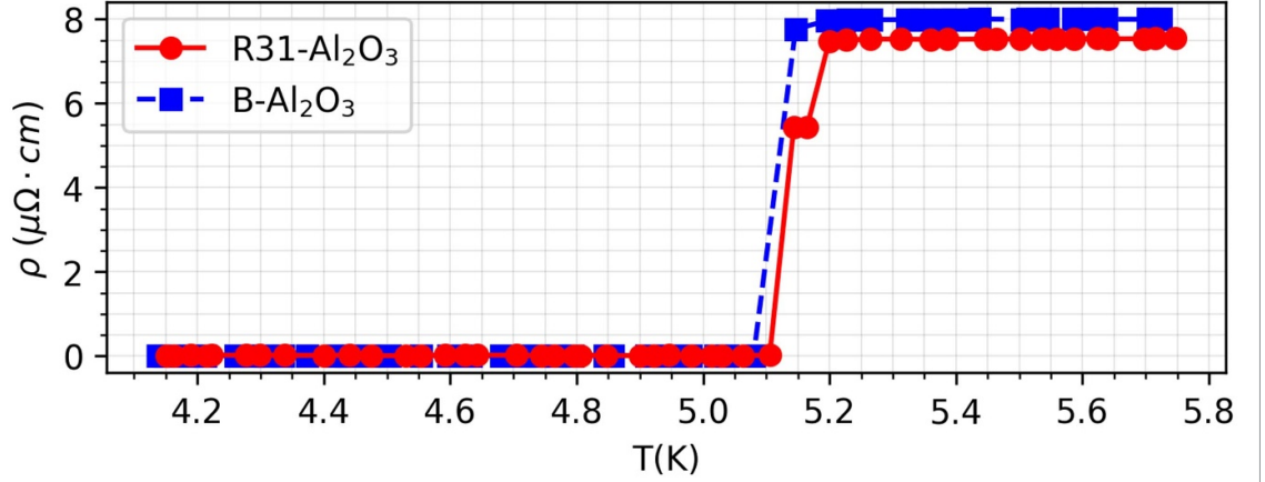
Figure C3. \rho(T) around the region of T_c for d = 106 nm thick TiN films grown on B- \text{Al}_2\text{O}_3 and R31- \text{Al}_2\text{O}_3 substrates.
