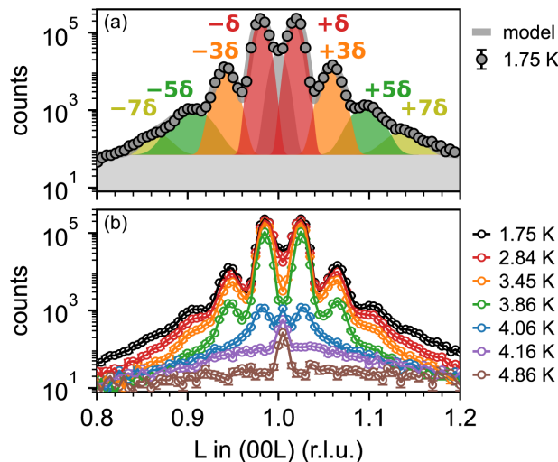
Figure 1 Neutron scattering intensities on the (00L) points in reciprocal space of single-crystal DyFeO 3 . They are shown on a logarithmic scale. (a) Representative scan at 1.75 K. Fits of odd magnetic satellite reflections up to seventh order are shown with coloured Gaussians, and the background is shown with a grey rectangle. (b) Selected scans in the temperature range 1.75–4.86 K.
