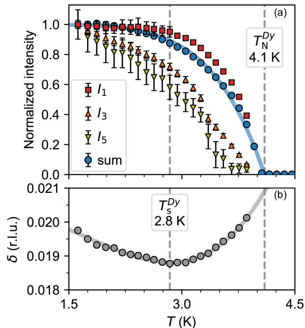
Figure 2 Temperature dependence of key parameters describing the DyFeO 3 incommensurate magnetic ordering. (a) Normalized integrated intensities of the sum and first- ( I_1 ), third- ( I_3 ) and fifth-order ( I_5 ) satellite reflections. (b) Modulation vector (0, 0, \delta ) length. The saturation temperature of the first-order satellites, T_s^{\text{Dy}} = 2.8 K, corresponds to the minimum of the modulation vector length \delta = 0.0187 (1) r.l.u. Note that the intensities of the third- and fifth-order satellite reflections are not saturated down to the lowest temperatures measured.
