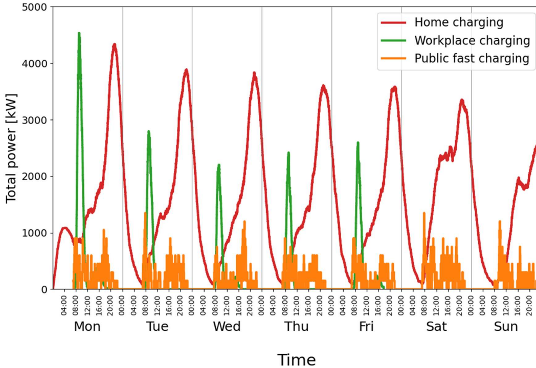
Figure 2: Weekly profile of the total power demand to charge electric vehicles, differentiated according to the charging locations.
