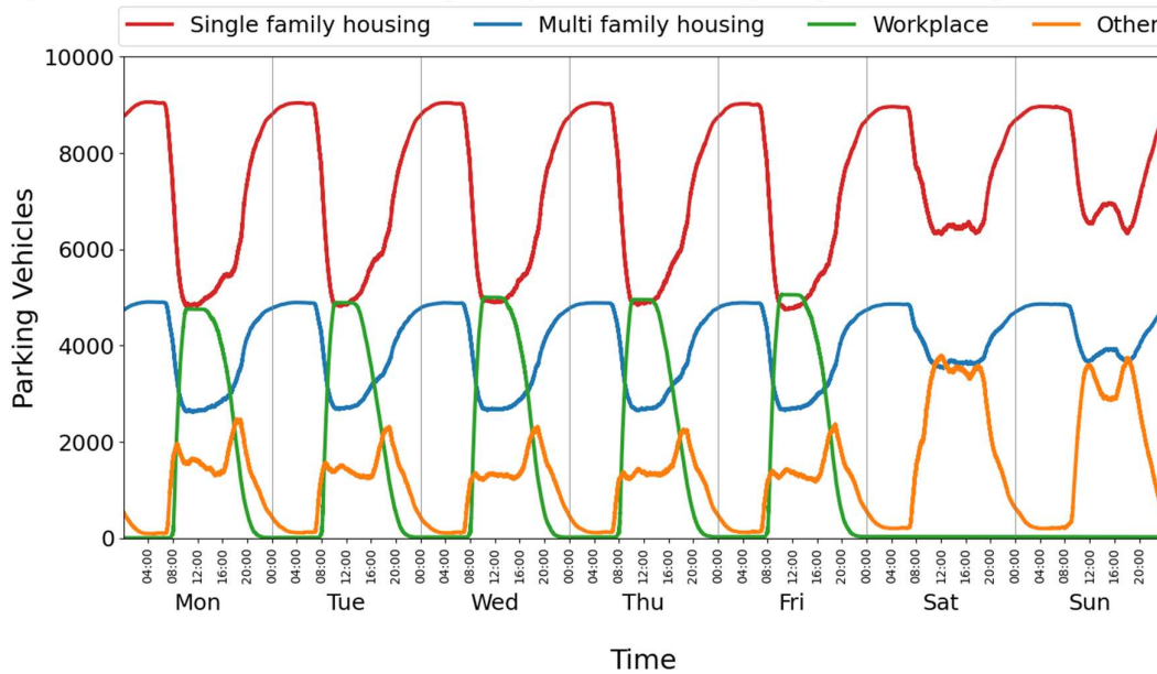
Figure 1: Parking locations of the electric vehicles for the city of Jülich, Germany over the course of a week.
