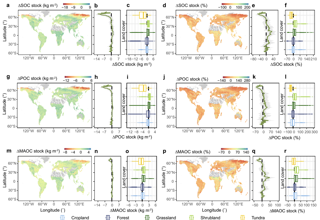
Fig. 3 | Global changes in soil organic carbon (SOC) stock, particulate organic carbon (POC) stock, and mineral-associated organic carbon (MAOC) stock under SSP 585 scenario. a, d, g, j, m, p Global distribution of the absolute and relative change of topsoil SOC, POC, and MAOC stocks under SSP585 scenario from 2081 to 2100. SSP, shared socioeconomic pathway. Here, SOC stock represents the sum of POC and MAOC stocks. \Delta POC, \Delta MAOC, and \Delta SOC stocks are the differences between the future and present stocks. The POC and MAOC stocks from 2081 to 2100 were calculated using climatic factors of different models under SSP585 scenario. The future mean annual temperature, mean annual precipitation, temperature seasonality, precipitation seasonality, evapotranspiration, and leaf
