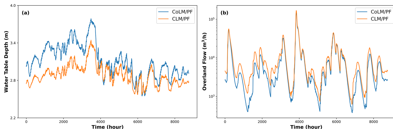
Figure 5. Panels (a) and (b) show the simulated water table depth and overland flow by CoLM/ParFlow and CLM/ParFlow, respectively. Each subplot represents spatial averages over the entire modeling domain.
