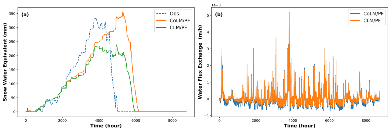
Figure 4. Panel (a) shows the simulated snow water equivalent from the CoLM/ParFlow and CLM/ParFlow single column models, compared against SNOTEL observations. Panel (b) presents the spatially averaged net water fluxes from CoLM and CLM to ParFlow, representing the source and sink terms in the ParFlow domain; both fluxes represent spatial averages over the entire modeling domain.
