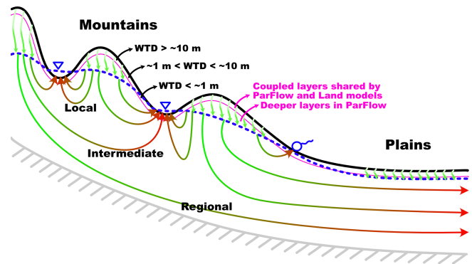
Figure 1. Illustration of the lateral groundwater flow, the critical zone of water table depth, and the coupling strategy between ParFlow and land surface models. Modified from Yang et al. (2023).
