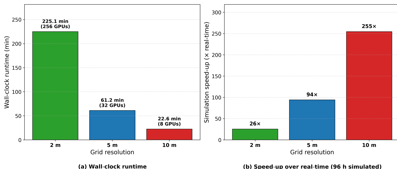
Figure 7. Computational performance of the SERGHEI simulations at dx = 2, 5 , and 10 m resolutions on the JUWELS Booster module (NVIDIA A100-SXM4-40GB GPUs). (a) Wall-clock runtime in minutes, and number of GPUs used for each configuration. (b) Simulation speed-up over real time, defined as the ratio of the simulated event duration (96 h) to the wall-clock runtime.
