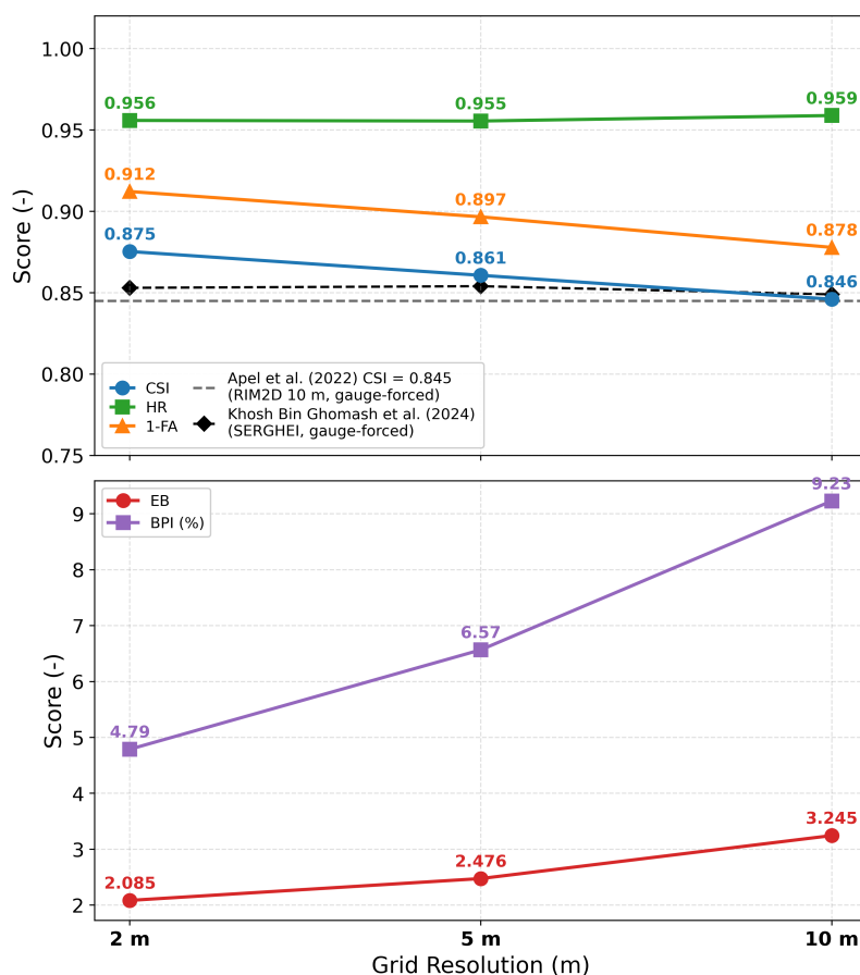
Figure 3. Flood extent performance metrics against the observed flood map, shown as a function of grid resolution. Skill scores of CSI = Critical Success Index, HR = Hit Rate, and 1–FA = 1 – False Alarm ratio, EB = Error Bias and BPI = Bias Percentage Indicator are presented. Metrics were calculated within a 1 km buffer along the main Ahr river channel using a minimum water depth threshold of 0.10 m. The horizontal dashed line marks the CSI of 0.845 reported by Apel et al. (2022) for the gauge-forced RIM2D setup of the lower Ahr Valley, and the dashed line with diamond markers shows the resolution-specific CSI values of Khosh Bin Ghomash et al. (2024) for the gauge-forced SERGHEI setup of the lower Ahr Valley.
