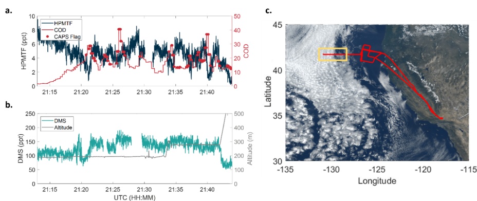
Figure 2. Time series of chemical measurements from the DC-8, taken during research Flight 3 (June 21, 21:00–22:00, 2023). 1-s time resolution of (a) HPMTF mixing ratio (dark-blue trace), cloud optical depth (COD, red trace), and instances when the CAPS detects a cloud droplet (red circles), (b) DMS mixing ratio (green trace), DC-8 altitude (gray trace). (c) True color image of flight path during AEROMMA June 21st 2023; yellow box indicates area highlighted in panels (a) and (b).
