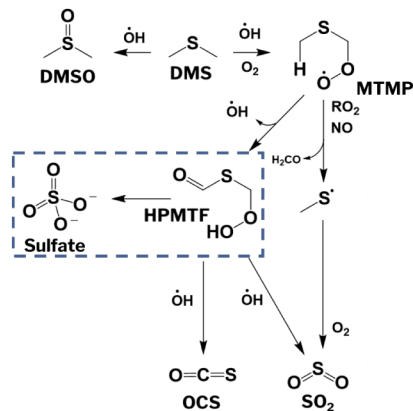
Figure 1. Simplified chemical mechanism for the gas-phase OH oxidation of dimethyl sulfide (DMS) and hydroperoxymethyl thioformate (HPMTF). Reaction products include methyl thiomethyl peroxy radical (MTMP), dimethyl sulfoxide (DMSO), sulfur dioxide ( \text{SO}_2 ), carbonyl sulfide (OCS), and sulfate ( \text{SO}_4^{2-} ). The segmented box highlights simplified aqueous HPMTF reactions forming sulfate.
