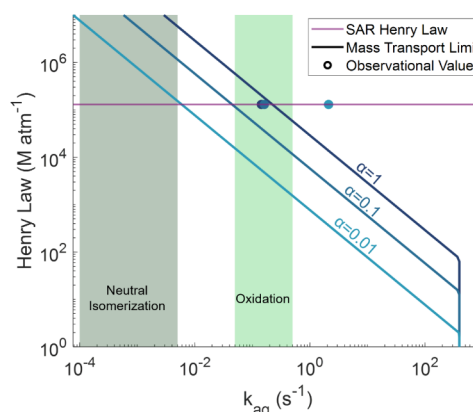
Figure 4. Range in overall first-order aqueous loss rate constant of HPMTF ( k_{\text{aq}}, \text{s}^{-1} ) as a function of a range of Henry's law coefficients. The purple line represents the approximated Henry's law coefficient for HPMTF using a structure activity relationship ( 1.3 \times 10^5 \text{ M atm}^{-1} ). The blue traces represent the maximum first-order aqueous loss rate given mass-transport limitations of HPMTF to the droplet at a given mass accommodation value with the darker and lighter hues representing the upper bound (1) and lower bound (0.012), respectively. The shaded regions provide ranges of hydroperoxy-aldehyde isomerization values in neutral solution (dark green) and DMS oxidation by ozone and hydrogen peroxide (light green). Median retrieved overall first-order aqueous loss rate constant of HPMTF at a Henry's law constant of 1.3 \times 10^5 and mass accommodation of 1, 0.1, and 0.012 are presented as circles of darker to lighter hues of blue, respectively. All points are calculated using an average cloud droplet diameter of 10 \mu\text{m} .
