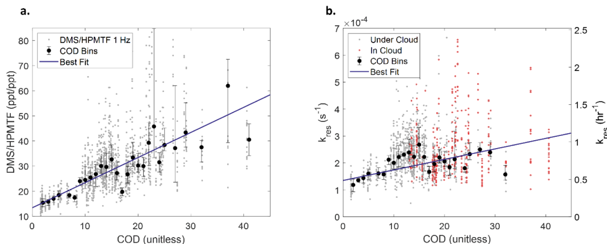
Figure 3. (a) 1-s resolution (gray), median (black dot), and interquartile range (error bar) of the DMS/HPMTF ratio values during the time under cloud, binned by whole cloud optical depth (COD) values. The blue line represents a best fit of the observations using a linear ODR ( R^2 = 0.76 ). (b) 1-s-resolution observations of the calculated k_{res} (using eq 2) at varying COD. Observations are separated by under-cloud (gray) or in-cloud (red) using the CAPS probe. Median under-cloud and in-cloud binned observations (black circles), interquartile ranges (error bars), and an ODR best fit (blue line, R^2 = 0.55 ) are calculated using the same bins as (a).
