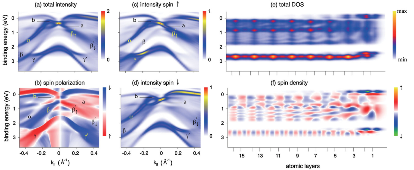
FIG. 3 (color). (a)–(d) Theoretical energy-momentum distribution of photoemission intensity for \mathbf{k}_{\parallel} along the \bar{\Gamma}\bar{M} line of SBZ. (a) spin-integrated intensity, (b) spin polarization, (c) spin- \uparrow , and (d) spin- \downarrow intensities. (e),(f) Local depth-resolved k_{\parallel} projected DOS \rho_{\mathbf{k}_{\parallel}}(z, E) for k_{\parallel} = 0.2 \text{ \AA}^{-1} : (e) total DOS (arb. units), (f) spin density \rho_{\mathbf{k}_{\parallel}}^{\uparrow} - \rho_{\mathbf{k}_{\parallel}}^{\downarrow} . One-half of the slab is shown, vacuum is to the right. Tics in the horizontal axis show the positions of atomic layers.
