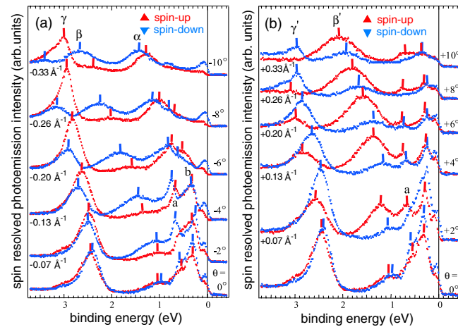
FIG. 1 (color online). Spin-resolved EDCs for Bi(111) surface from 0 to 3.7 eV binding energy, (a) from \theta = 0^\circ to -10^\circ and (b) from \theta = 0^\circ to +10^\circ . Corresponding wave numbers are presented for every EDC on the left side of each frame.
