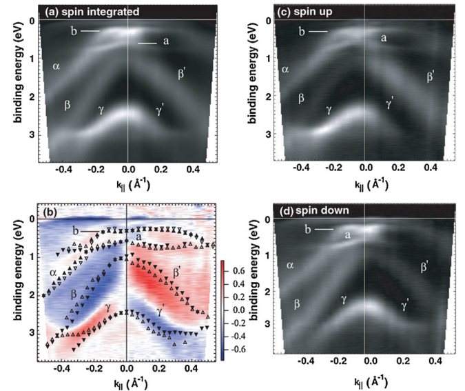
FIG. 2 (color). Experimental photoemission intensity distribution for k_{\parallel} in \bar{\Gamma}\bar{M} direction. (a) spin-integrated intensity I(E, k_{\parallel}) . (b) spin polarization P(E, k_{\parallel}) = (I_{\uparrow} - I_{\downarrow})/(I_{\uparrow} + I_{\downarrow}) : positive (negative) polarization is plotted in red (blue); color strength gives the absolute value of P(E, k_{\parallel}) . (c) spin-up I_{\uparrow} and (d) spin-down I_{\downarrow} intensities. Intensity maxima of spin- \uparrow (spin- \downarrow ) EDCs are plotted with open (filled) triangles in graph (b).
