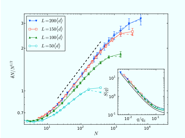
Fig. 5: (Colour online) Number fluctuations \delta N/N^{1/2} versus N for different system sizes L , and two different procedures P1 and P2 corresponding to time-averaging first (P1, solid lines) and spatial-averaging first (P2, dashed lines). K/K_0 = 5 \times 10^{-5} , \eta/\eta_0 = 0.24 , and the dashed line has a slope of 0.31. (Inset) Static structure factor S(q) for the same systems, with q_d = 2\pi/\langle d \rangle . The solid line corresponds to S(q) \propto q^{-1.8} + B .
