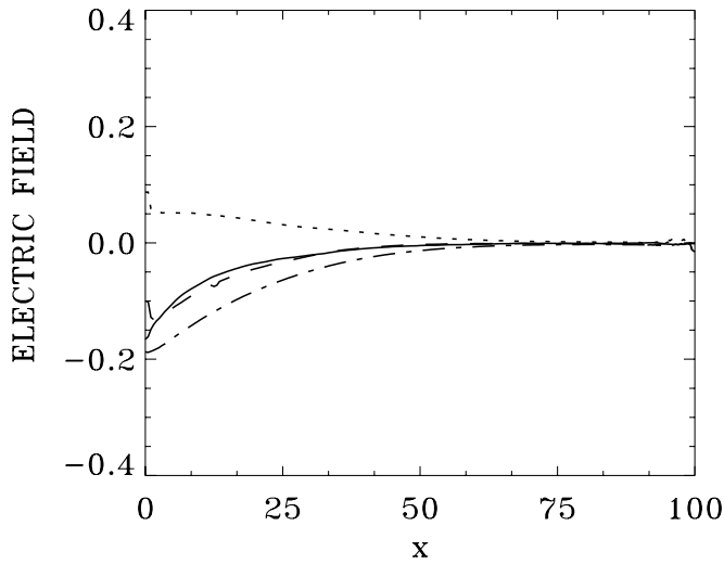
FIG. 21. Electric field at t=315 (full curve), \nabla P_i/n_i (dotted curve), 0.1\langle v_z \rangle/\cos \alpha (dash-dot curve), and \nabla P_i/n_i + 0.1\langle v_z \rangle/\cos \alpha (dash curve).
