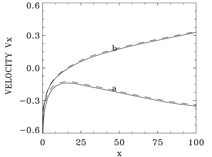
FIG. 16. Velocity \langle v_x \rangle at (a) t=370 and (b) t=420 (ions full curves, electrons broken curves \langle v_x \rangle \sin \alpha ).
