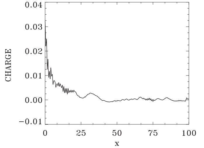
FIG. 31. Charge ( n_i - n_e ) at t=213 .
