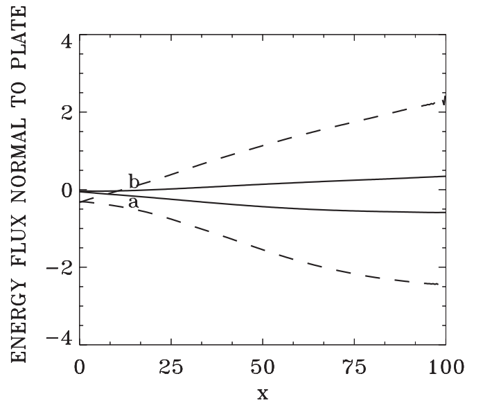
FIG. 7. Energy flux normal to plate ( Q_e full curves, Q_i dash curves) at (a) t=375 and (b) t=425 .
