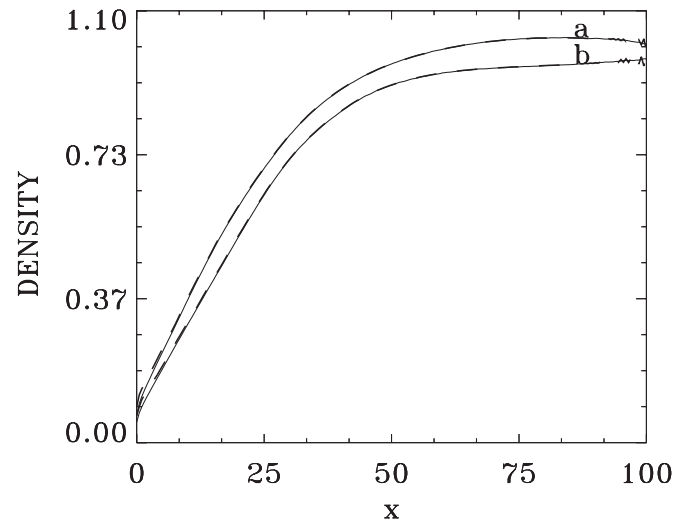
FIG. 24. Density profiles (full curve electrons, broken curve ions) at (a) t=290 and (b) t=340 .
