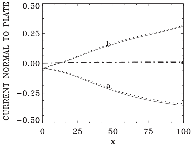
FIG. 5. Current normal to plate (full curve electrons, dotted curve ions) at (a) t=375 and (b) t=425 (the dash-dot curve is the total current, essentially zero).
