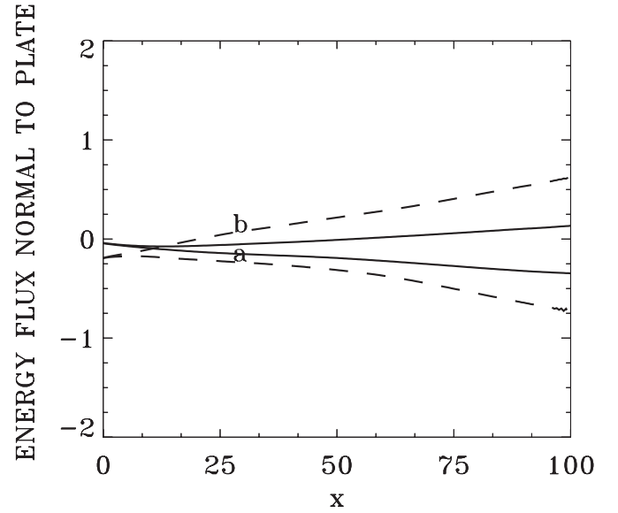
FIG. 23. Energy flux normal to the plate ( Q_e full curves, Q_i dash curves) at (a) t=375 and (b) t=425 .
