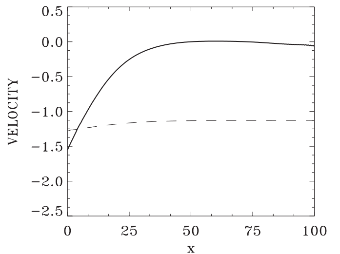
FIG. 36. Velocity at t=213 (dash curve \langle u_y \rangle , full curve \langle u_z \rangle ).
