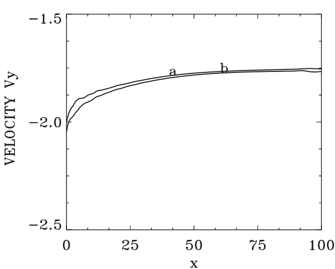
FIG. 26. Velocity \langle v_y \rangle at (a) t=265 and (b) t=315 .
