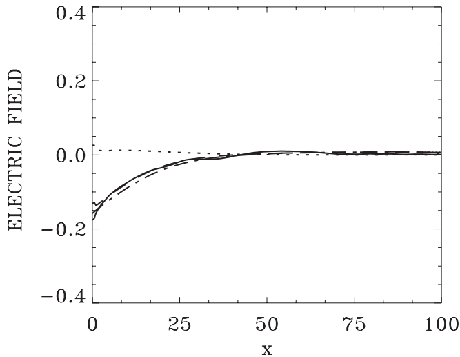
FIG. 30. Electric field at t=213 (full curve), \nabla P_i/n_i (dotted curve), 0.1\langle v_z \rangle/\cos \alpha (dash-dot curve), and \nabla P_i/n_i + 0.1\langle v_z \rangle/\cos \alpha (dash curve).
