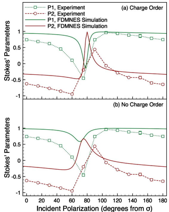
FIG. 13. (Color online) Comparison between the experimental and simulated polarization dependencies for the (-\frac{1}{2}, 3, 7) reflection (a) with and (b) without charge ordering, with both simulations at 7.1227 keV (on-resonance).
