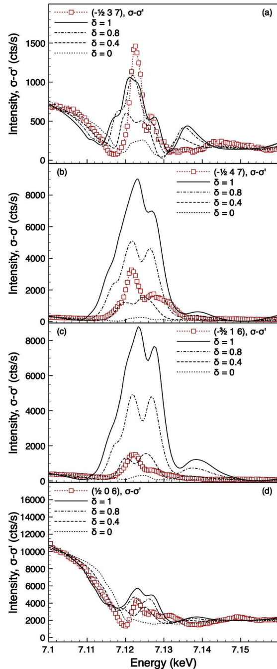
FIG. 12. (Color online) Experimental spectra and simulations at 220 K, of the (a) (-\frac{1}{2}, 3, 7) , (b) (-\frac{1}{2}, 4, 7) , (c) (-\frac{3}{2}, 1, 6) , and (d) (\frac{1}{2}, 0, 6) reflections, showing the effect of charge disproportionation on the resonance. The simulations use the diagonal structure and apply iron valences of +2.5 \pm \frac{\delta}{2} . The simulation has been corrected to include absorption.
