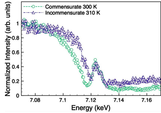
FIG. 7. (Color online) Energy scans of the (-\frac{1}{2}, 3, 7) and (-\frac{1}{2}, 3, 7 + \tau) reflections in the \sigma - \sigma' channel, measured at fixed wave vector. The spectra have been normalized to the low-energy off-resonance intensities.
