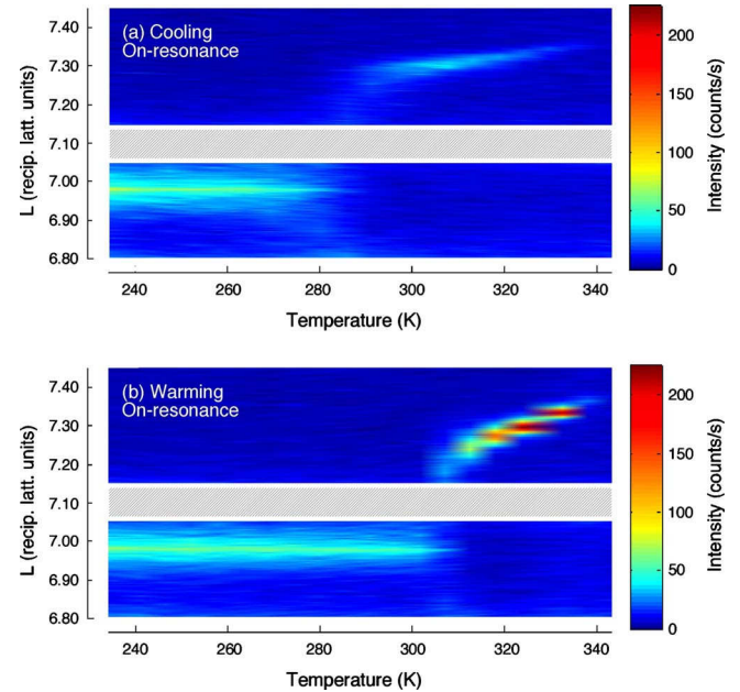
FIG. 8. (Color online) Temperature dependence on (a) cooling and (b) warming of the (-\frac{1}{2}, 3, 7) and (-\frac{1}{2}, 3, 7 + \tau) reflections in the \sigma - \sigma' channel, measured on-resonance at 7.123 keV [see the marked position in Fig. 5(a)]. The sample was cooled/warmed at a rate of 0.2 K/min. The hashed area contains contamination from a powder reflection.
