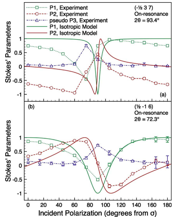
FIG. 11. (Color online) Linear polarization analysis of the (-\frac{1}{2}, 3, 7) and (\frac{1}{2}, -1, 6) reflections, measured at 220 K, on-resonance. The solid lines show the behavior expected for isotropic charge scattering.
