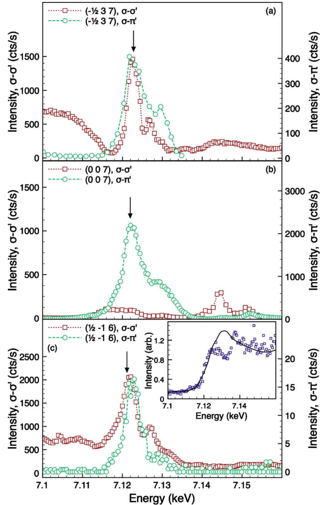
FIG. 5. (Color online) Energy scans of several reflections, measured at fixed wave vector at 220 K. The arrows mark the resonant energies at which full linear polarization analysis was undertaken. Full linear polarization analysis was also undertaken well below the absorption edge for (a) and (c). Inset. The measured (symbols) and simulated (solid line) fluorescence spectrum used for energy calibration.
