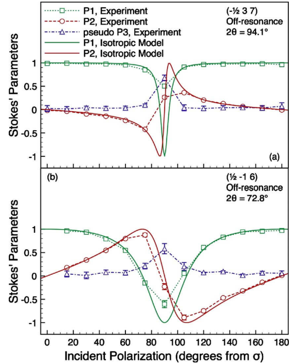
FIG. 10. (Color online) Linear polarization analysis of the (-\frac{1}{2}, 3, 7) and (\frac{1}{2}, -1, 6) reflections, measured at 220 K, off-resonance. The solid lines show the behavior expected for isotropic charge scattering.
