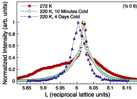
FIG. 4. (Color online) Scans along the L direction for the (\frac{1}{2}, 0, 6) reflection in the \sigma - \sigma' channel using an energy of 7.123 keV (on-resonance). The scan at 272 K was measured on cooling from the high-temperature phase, after cooling at a rate of 0.4 K/min. The scan at 220 K was measured after further cooling at the same rate. The final scan was measured after holding the sample at 220 K for 4 days.
