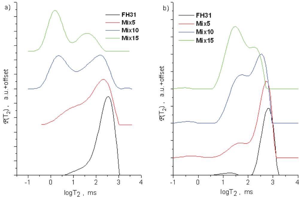
Fig.4.6. Distribution function \mathcal{F}(T_2) for saturated samples at a) B_0 = 7\text{T} and b) B_0 = 0.1\text{T} Data fitted according to eq.2.7 using 100 exponentially spaced T_2 values
