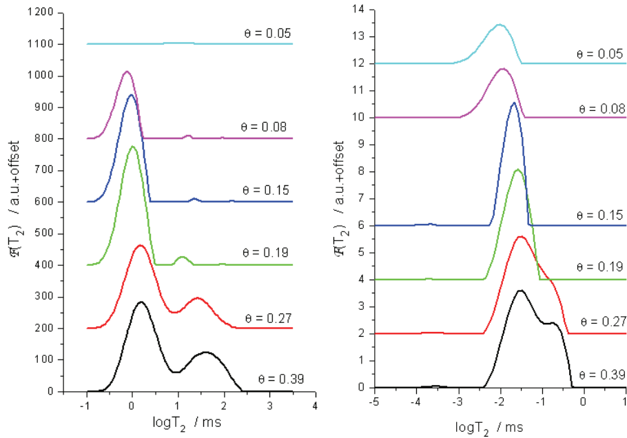
Distribution function F(T_2) for sample Mix15 at different water contents. a) B_0 = 7 T and b) B_0 = 0.1 T. Data fitted according to eq.2.7 using 100 exponentially spaced T_2 values
