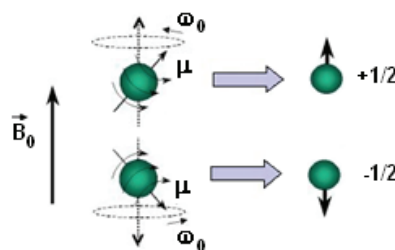
Fig.2.1. Particle with spin
