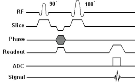
Fig.2.6. Spin-echo pulse sequence timing diagram
