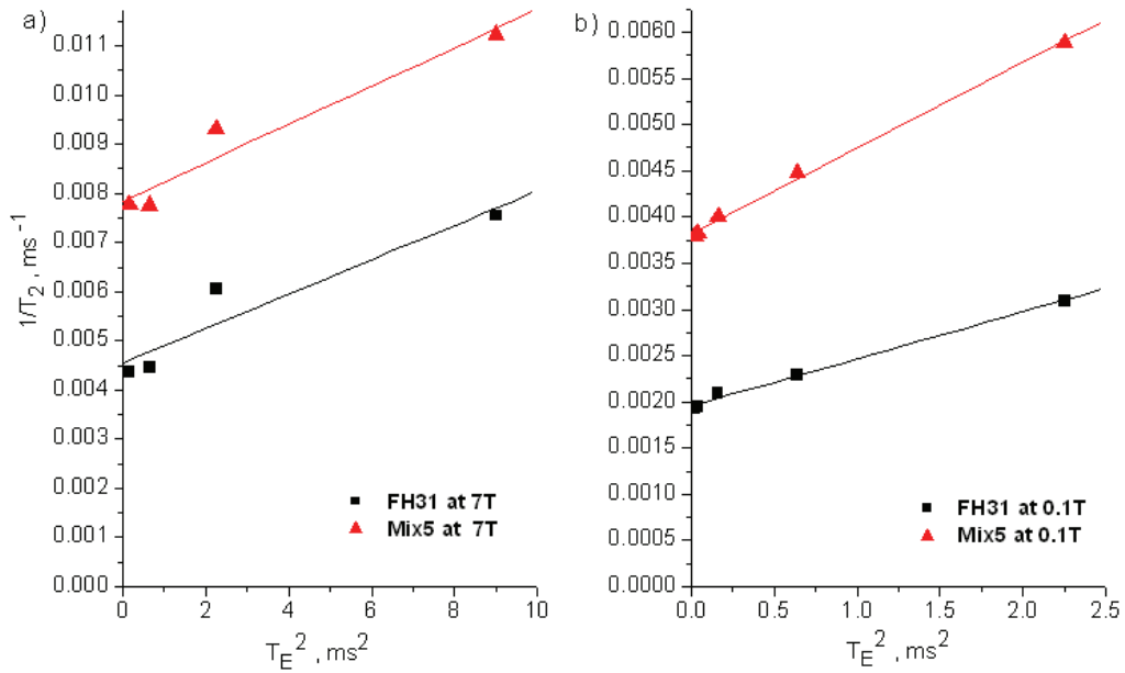
Fig.4.4. Estimation of diffusion influence: 1/T_2, \text{average} as a function of T_E^2 at a) 7T and b) 0.1T for two samples: FH31 saturated and Mix5 saturated. The field gradients were estimated using eq.2.11 to be 1.28 T/m for FH31 and 1.78 T/m for Mix5 in low magnetic field (right) and 1.089 T/m for FH31 and 1.13 T/m for Mix5 in high magnetic field (left)
