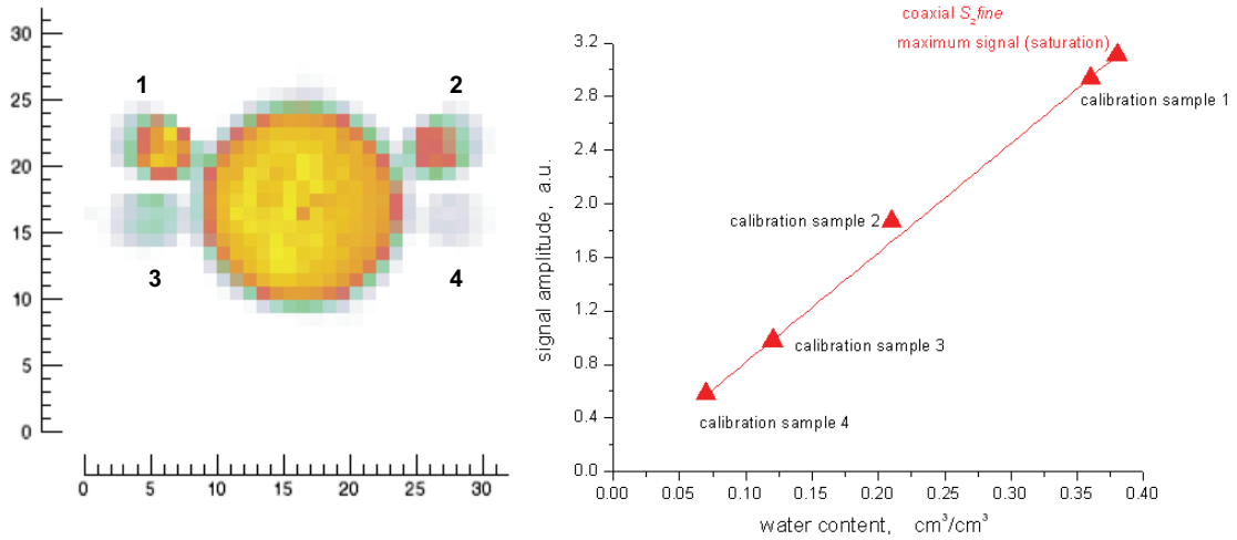
Fig.6.7.a) Reference image for the interpolation of the signal amplitude; axial central slice of the coaxial sample S2fine and calibration samples and b) Linear interpolation of the maximum MRI signal
