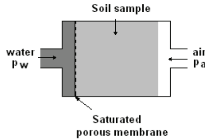
Fig.3.2. Idealized instrument for measuring soil water characteristic
