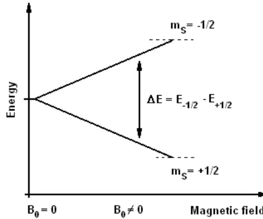
Fig.2.2. Energy difference between the nuclear spin levels
