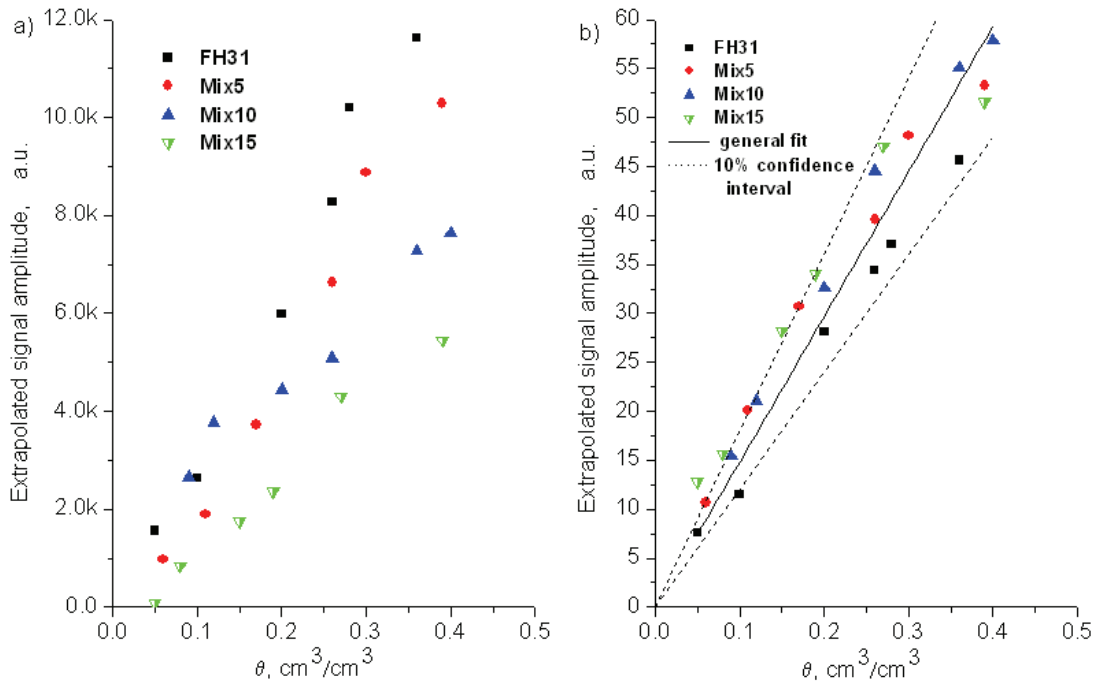
Fig.4.9. Extrapolated signal amplitudes at different mean volumetric water contents for all samples. a) B_0 = 7T and b) B_0 = 0.1T
