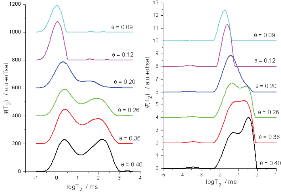
Distribution function F(T_2) for sample Mix10 at different water contents. a) B_0 = 7 T and b) B_0 = 0.1 T. Data fitted according to eq.2.7 using 100 exponentially spaced T_2 values
