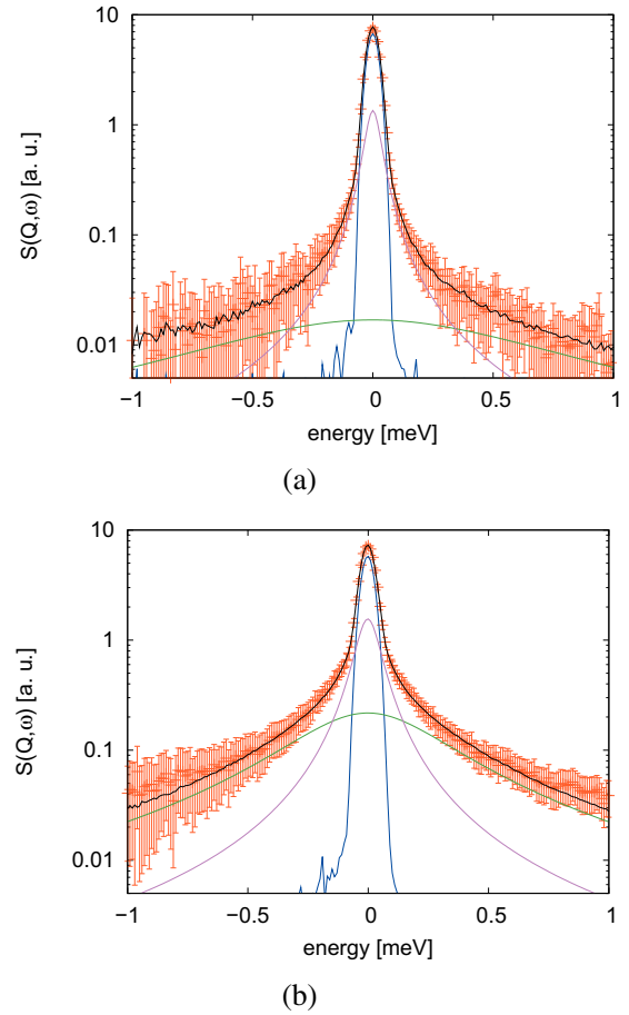
FIG. 3. Plot of S(\vec{Q}, \omega) for (a) Q=0.44 \text{ \AA}^{-1} and (b) Q=1.48 \text{ \AA}^{-1} at 5 \text{ }^{\circ}\text{C} . The resulting fit is shown (black line) as well as the single contributions. The delta function is drawn in the blue line; the two Lorentzians are plotted as green and pink lines, respectively.
