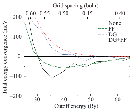
FIG. 2. (Color online) Convergence of total energy for Cu atom as a function of the coarse-grid cutoff energy \pi^2/H^2 (Ry). Zero total energy is set at that computed with cutoff energy of 67 Ry.
