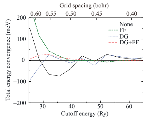
FIG. 3. (Color online) Total-energy variation E - E' in Cu atom owing to egg box effect as a function of the coarse-grid cutoff energy \pi^2/H^2 (Ry). Here, E is the total energy when the atom is located at the center between adjacent coarse-grid points and E' is the energy when the atom is shifted by 0.5H_x along the x direction.
