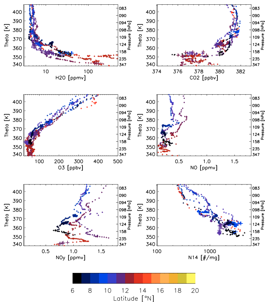
Fig. 10b Vertical profiles of trace gas concentrations (volume mixing ratio in ppbv or ppmv as appropriate) and aerosol mass mixing ratio (particles per mg air), N_{14} (14 nm to <1\ \mu\text{m} ), for “non-convective” M55 flights on 4 and 13 August 2006. Profiles are plotted as a function of theta (K) and coloured by latitude where the measurements were made. Crosses indicate points where back trajectories show uplift from below 800 hPa during 10 days before the flight.
