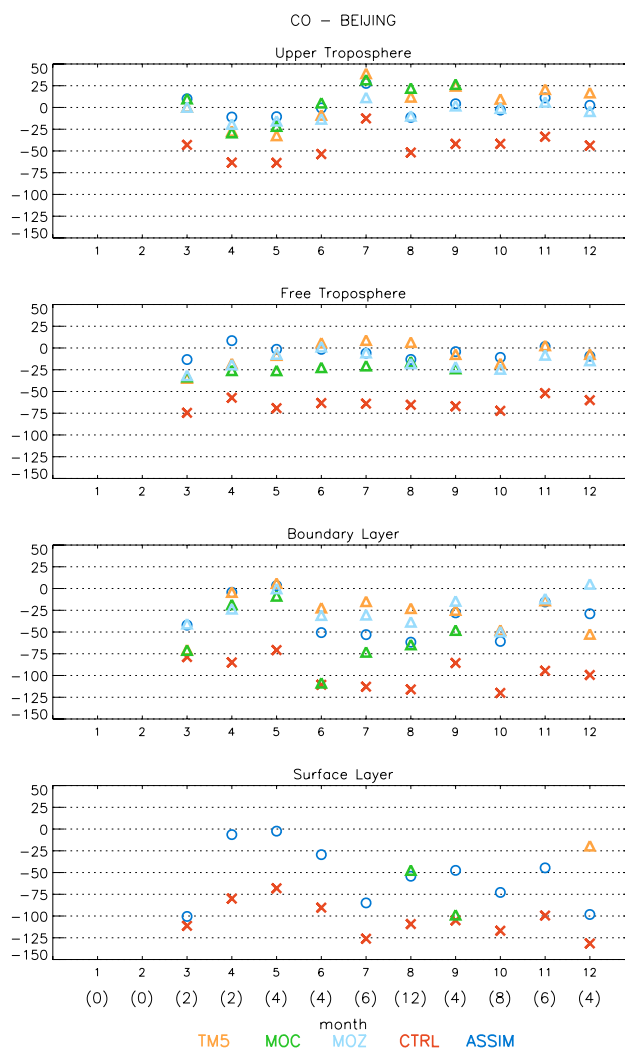
Fig. 6. Same as Fig. 5 except over Beijing.
