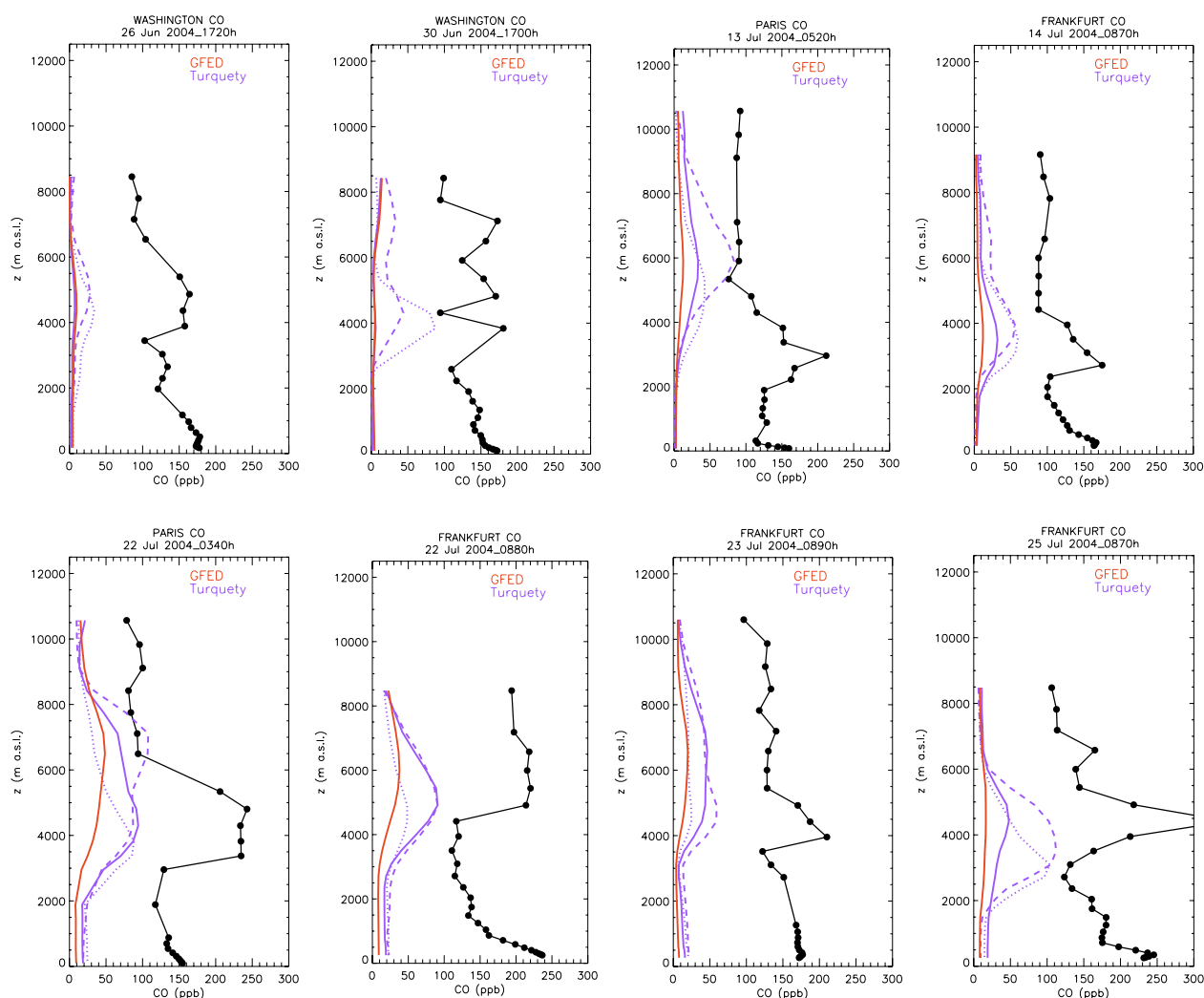
Fig. 12. Vertical profiles of modelled tracer CO with GFED 8-day emissions (red line) and Turquety daily emissions (purple line) from biomass fires and observed CO (black line). Solid lines indicate tracers injected at the surface. Dotted and dashed lines represent the tracers injected at 6 and 8 km, respectively.
