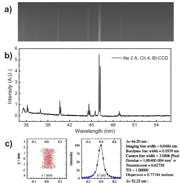
FIG. 2. (Color online) (a) Back-illuminated CCD image at Ch. 4 in Ne 2 A discharge, (b) spectrum with vertical binning of Back-illuminated CCD image, and (c) ray-tracing calculation result for the 44.50 nm line.
