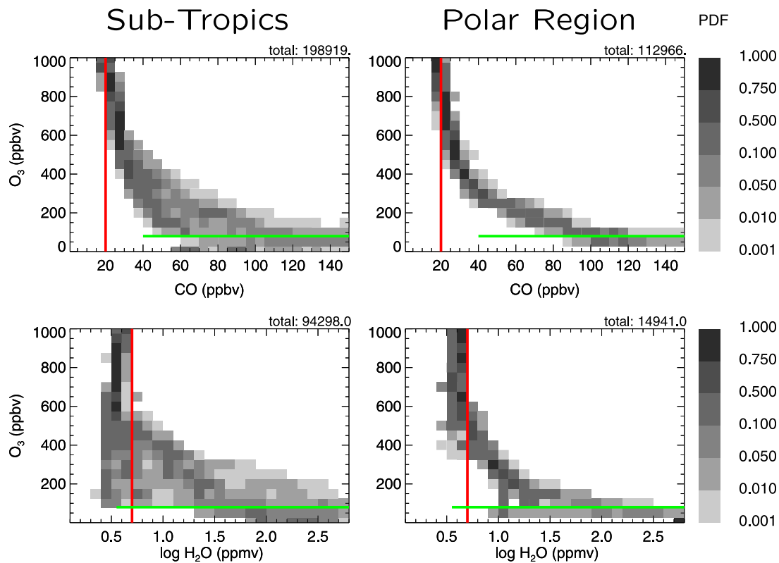
Figure 8. Probability distribution functions of (top) O_3 -CO correlations and (bottom) O_3 -H _2 O correlations derived from all aircraft observations for (left) subtropics and (right) the polar region in spring. Total number of data is given on the top right of each plot. The threshold for the stratospheric background values is shown in red and for the tropospheric background value in green (see text for more details). H _2 O is plotted on a logarithmic scale.
