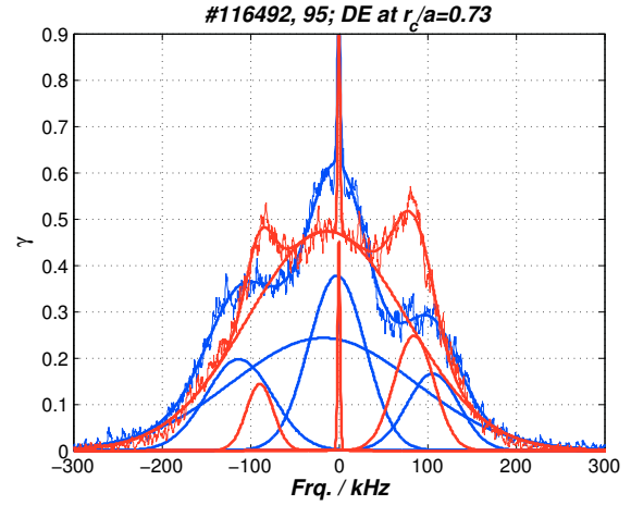
Figure 4: Same as for fig. 3 but for different r_c/a .
