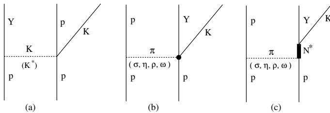
Fig. 1. Reaction mechanisms involving (a) strange, (b) non-resonant, and (c) resonant, non-strange meson exchange for pp \rightarrow pK^+Y , Y = \Lambda, \Sigma^0 . Initial and final state interactions are not indicated.
