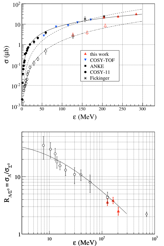
Fig. 4. Upper part: the world data set on total cross sections of pp \rightarrow pK^+\Lambda (solid symbols) and pp \rightarrow pK^+\Sigma^0 (open symbols) [1, 2, 3, 4, 5, 6, 7, 47]; dashed lines: phase space, solid line: phase space + FSI. Lower part: energy dependence of the cross section ratio R_{\Lambda/\Sigma^0} . The open diamond at \epsilon = 700 MeV is an average value calculated from the data given in [8]. The results of the present work are shown as triangles. The solid line is the ratio of the parametrizations of the two excitation functions.
