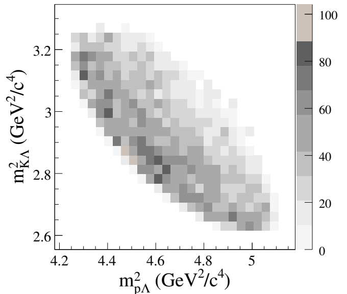
Fig. 5. Dalitz plot of the pK^+\Lambda final state measured at \epsilon = 204 \text{ MeV} . The data is acceptance corrected, however the background is not subtracted (see text). The scale of the relative bin occupancy is shown at the right side.
