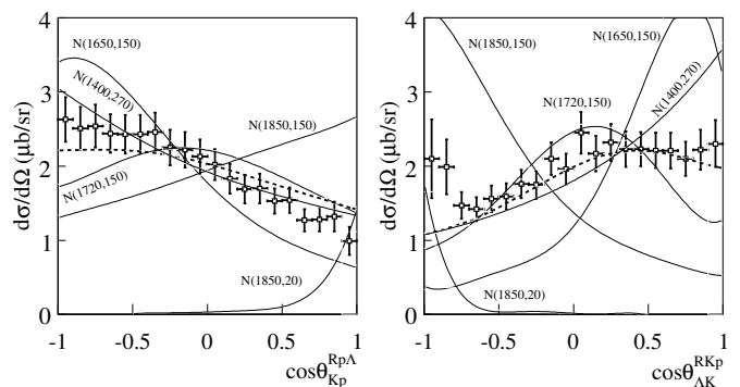
Fig. 9. Angular distributions measured in the p\Lambda and K^+ p helicity frames. The lines are the Monte Carlo result for various nucleon resonances ( N(m, \Gamma) ). The dashed line is the result for an incoherent sum of Monte Carlo data (see text).
