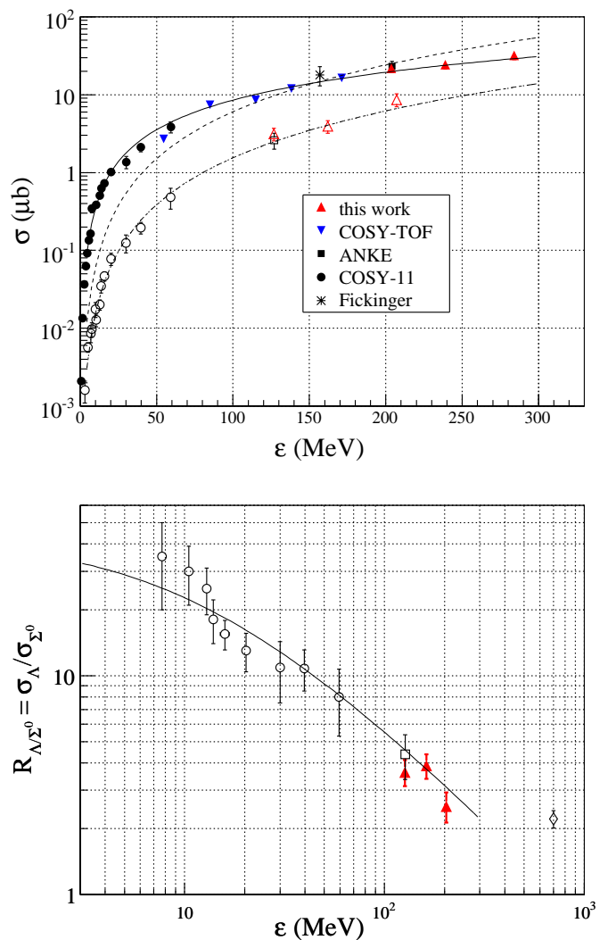
Fig. 4. Upper part: the world data set on total cross sections of pp \rightarrow pK^+\Lambda (solid symbols) and pp \rightarrow pK^+\Sigma^0 (open symbols) [1, 2, 3, 4, 5, 6, 7, 47]; dashed lines: phase space, solid line: phase space + FSI. Lower part: energy dependence of the cross section ratio R_{\Lambda/\Sigma^0} . The open diamond at \epsilon = 700 MeV is an average value calculated from the data given in [8]. The results of the present work are shown as triangles. The solid line is the ratio of the parametrizations of the two excitation functions.
