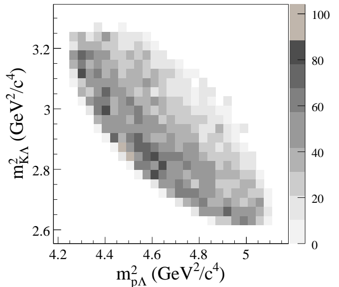
Fig. 5. Dalitz plot of the pK^+\Lambda final state measured at \epsilon = 204 \text{MeV} . The data is acceptance corrected, however the background is not subtracted (see text). The scale of the relative bin occupancy is shown at the right side.
