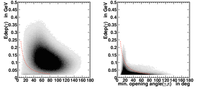
Figure 2: Correlation plot for laboratory photon energy vs charged track photon opening angle (Monte Carlo) (left:) signal, (right:) pd \rightarrow ^3\text{He} \pi^+ \pi^- reaction. The graphical cut to suppress pd \rightarrow ^3\text{He} \pi^+ \pi^- reaction is shown.
