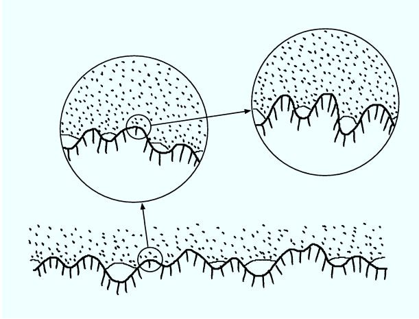
FIG. 6: An rubber block (dotted area) in adhesive contact with a hard rough substrate (dashed area). The substrate has roughness on many different length scales and the rubber makes partial contact with the substrate on all length scales. When a contact area is studied at low magnification it appears as if complete contact occur, but when the magnification is increased it is observed that in reality only partial contact occur.
