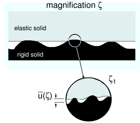
FIG. 7: An asperity contact region observed at the magnification \zeta . It appears that complete contact occur in the asperity contact region, but when the magnification is increasing to the highest (atomic scale) magnification \zeta_1 , it is observed that the solids are actually separated by the average distance \bar{u}(\zeta) .
