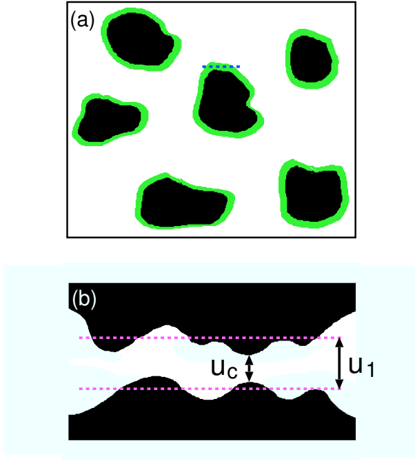
FIG. 8: (a) The black area is the asperity contact regions at the magnification \zeta . The green area is the additional contact area observed when the magnification is reduced to \zeta - \Delta\zeta (where \Delta\zeta is small). The average separation between the solid walls in the green surface area is denoted by u_1(\zeta) . (b) The separation between the solid walls along the blue dashed line in (a). Since the surfaces of the solids are everywhere rough the actual separation between the solid walls in the green area will fluctuate around the average u_1(\zeta) . At the most narrow constriction the surface separation is u_c .
