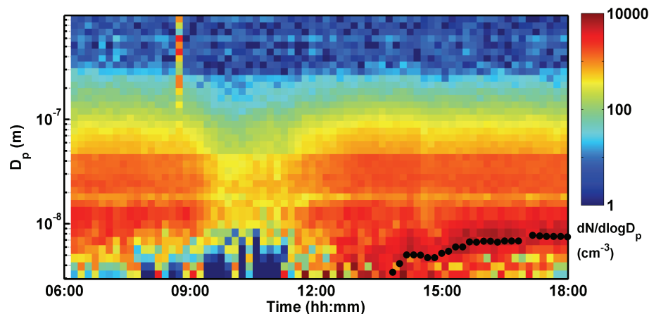
Fig. 8. The contribution of low-volatility material to the nucleation mode growth in Hyytiälä during an atmospheric nucleation event on 15 April 2007. The particle size distributions measured with the V-DMPS system after the ambient aerosol sample has been heated to 280 °C. The black dots represent the geometric mean size of the growing nucleation mode after heating.
