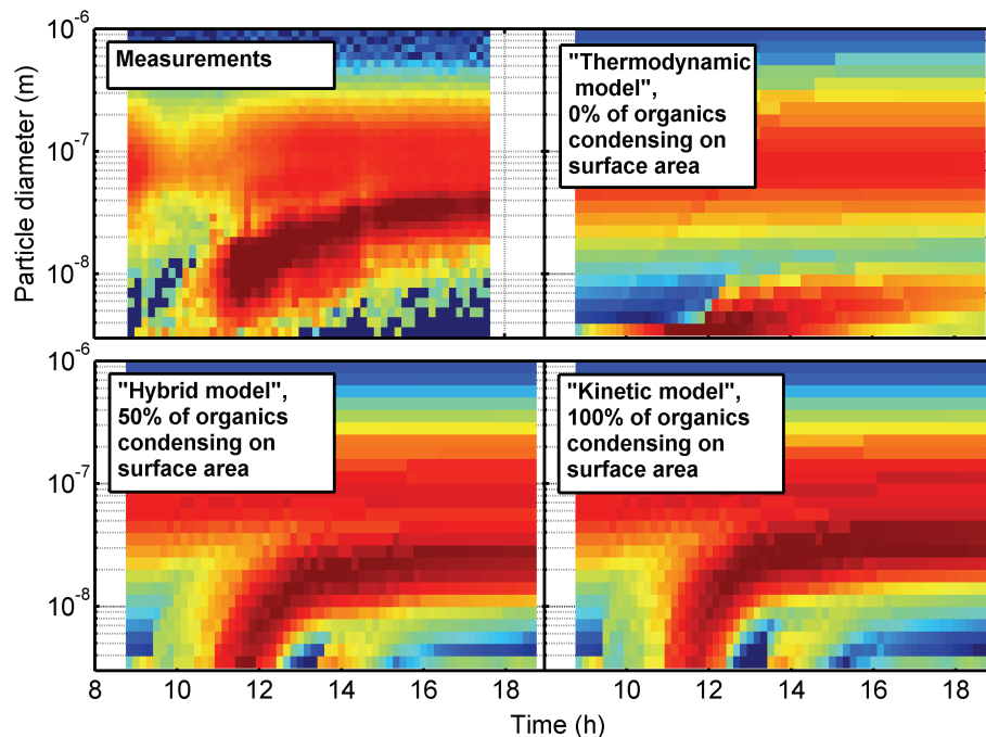
Fig. 5. A comparison between the evolution of the atmospheric size distribution on 15 April 2007 in Hyytiälä (A) with the box model calculations assuming 0% (B) ; 50% (C) ; 100% (D) of the organic mass to condense on the aerosol surface area. In panel (B) only sulfuric acid is condensing on the surface area of the aerosol – the organics are distributed to the pre-existing mass.
