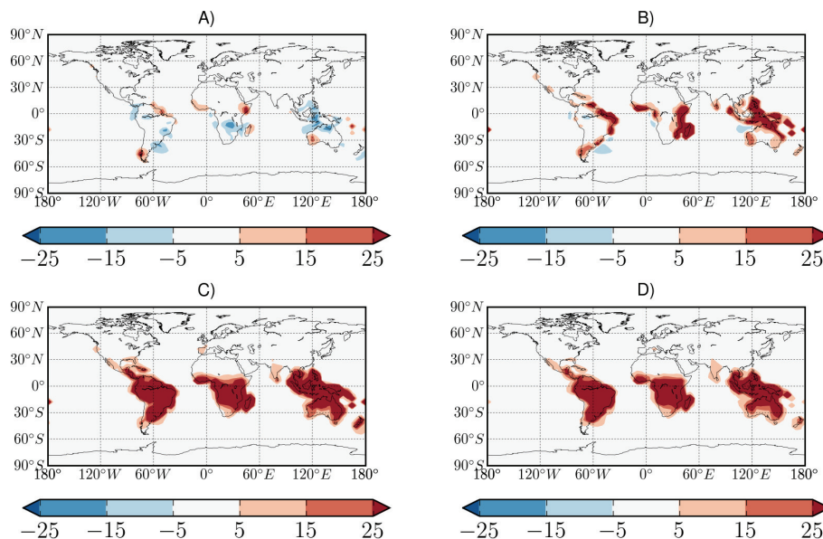
Fig. 11. Increases in aerosol number concentrations due to ultrafine aerosol growth by fully kinetic approach as compared with the semi-empirical scheme for June 2001. Changes in global aerosol number concentrations (average over 1 km) if all of the total OA mass is distributed as effectively non-volatile, as compared with the case where 50% of it partitions to the pre-existing aerosol mass. The colorscale indicates percentage changes in number concentrations of particles >3 nm (A), >10 nm (B), >40 nm (C), and >80 nm (D).
