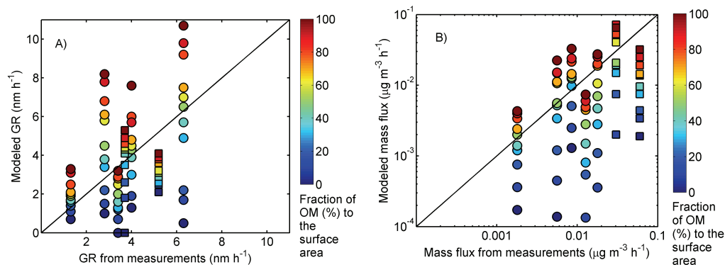
Fig. 7. Particle growth rates (A) and mass fluxes (B) as determined from the measurement data and the model simulations for 7 particle formation event days in Hyytiälä and Egbert (see Table 2). The color scale depicts the fraction of total OA mass flux that was distributed on aerosol surface area in each of the simulations.
