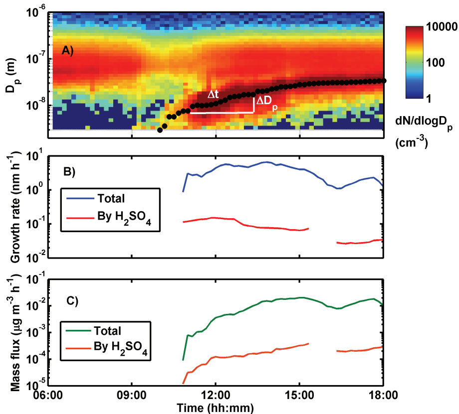
Fig. 2. Aerosol formation and growth event on 15 April 2007 at the SMEAR II station in Hyttiälä, Finland. (A) Evolution of aerosol number size distribution. The black dots represent the geometric mean size of the nucleation mode. (B) Particle diameter growth rate ( \text{GR} = \Delta D_p / \Delta t ) and (C) Mass flux to the nucleation mode as determined from the data and calculated based on ambient sulfuric acid concentrations. The GR and mass flux by sulfuric acid are theoretical maximum values.
