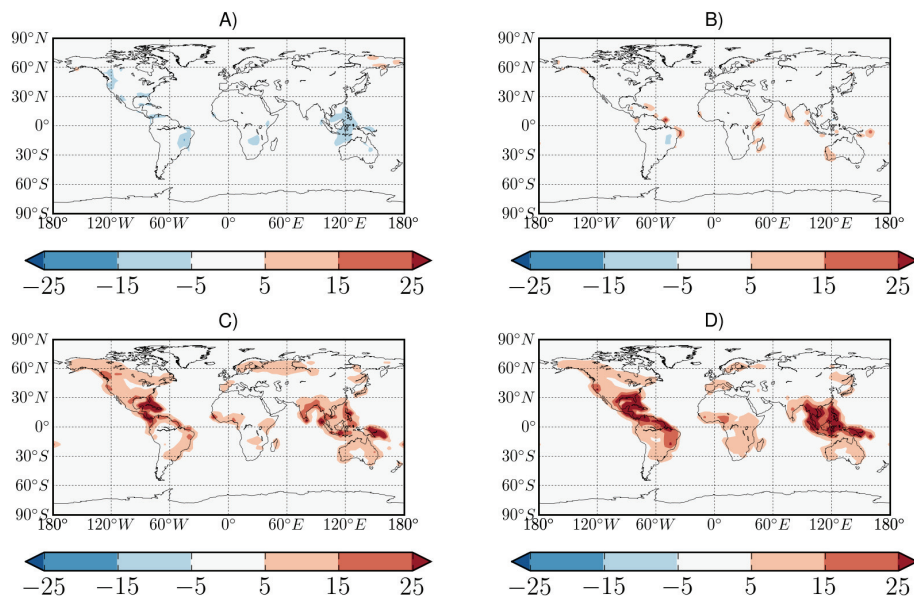
Fig. 10. Increases in aerosol number concentrations due to ultrafine aerosol growth by semi-empirical organic condensation scheme for March 2001. Changes in global aerosol number concentrations (average over 1 km) if 50% of the total OA mass is distributed as effectively non-volatile, as compared with the case where is partitions to the pre-existing aerosol mass. The colorscale indicates percentage changes in number concentrations of particles >3 nm (A) , >10 nm (B) , >40 nm (C) , and >80 nm (D) .
