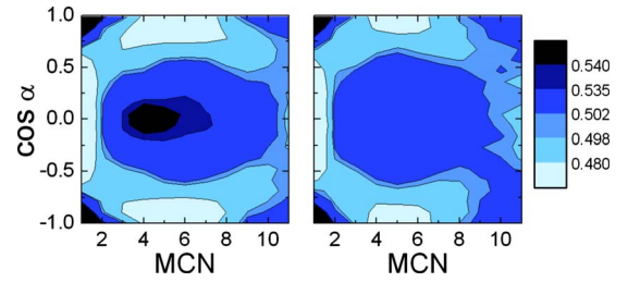
FIG. 2. (Color online) Short-range order for the HDL (left) and the LDL (right), at 230 and 280 \text{ K} , respectively. The y axis is the cosine of the angle \alpha formed between the vectors defined by the C–C double bonds of two neighbor molecules and the x axis is the number of molecules surrounding a central one. The z axis represents the probability of finding two molecules at a distance determined by the MCN with a relative orientation defined by the \alpha angle.
