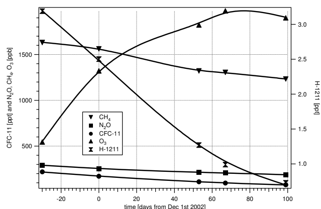
Fig. 4. Averages of tracers at the 400 K isentrope in the vortex versus the time ( \chi_{\text{vortex}}(t) ). The data were fitted with a smoothing spline. Points refer to measurements made during Geophysica campaigns and the MKIV flight.
