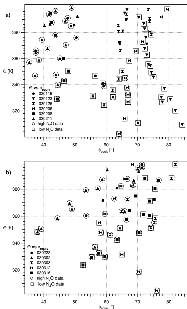
Fig. 10. Potential temperature plotted versus equivalent latitude. (a) Data of the EuPLEX Campaign, (b) data of the AVC campaign. The “low N 2 O data” are highlighted by black squares and the “high N 2 O data” are highlighted by black circles.
