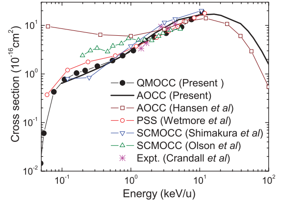
FIG. 13. (Color online) Total nonradiative charge-transfer cross sections for \text{B}^{3+}(1s^2) + \text{H}(1s) collisions. Shown are present QMOCC results (solid line with filled circles); present AOCC results (solid line); AOCC results of Hansen et al. [7] (solid line with open squares); PSS results of Wetmore et al. [4] (solid line with open circles); SC-MOCC results of Shimakura et al. [6] (solid line with downward triangle); SC-MOCC results of Olson et al. [5] (solid line with upward triangle); and experiment results of Crandall et al. [10] (stars).
