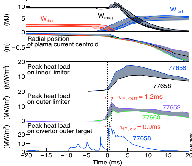
Fig 5 (a) the thermal, W_{th} , magnetic, W_{mag} and radiated, W_{rad} energies during the 40ms around the thermal quench ( t=0 ). (b) the radial position of the current centroid with respect to the major radius, R_0 . (c) to (e) the peak heat load measured on the inner limiter, outer limiter and outer target of the divertor respectively.
