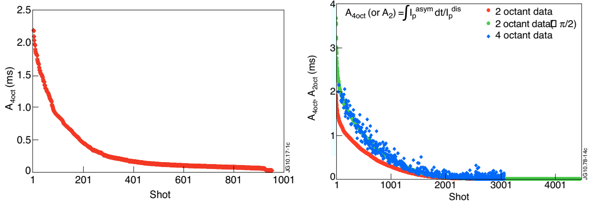
Fig 1 Left-hand plot shows A_{4\text{ oct}} for the whole 4 octant database (with data sorted into descending order). The right-hand plot shows the entire 2 octant database (red), data for 4 octant shots (blue) where it exists, and \pi/2 A_{2\text{ oct}} (green). In the right-hand plot the data are sorted by descending size of A_{2\text{ oct}}
