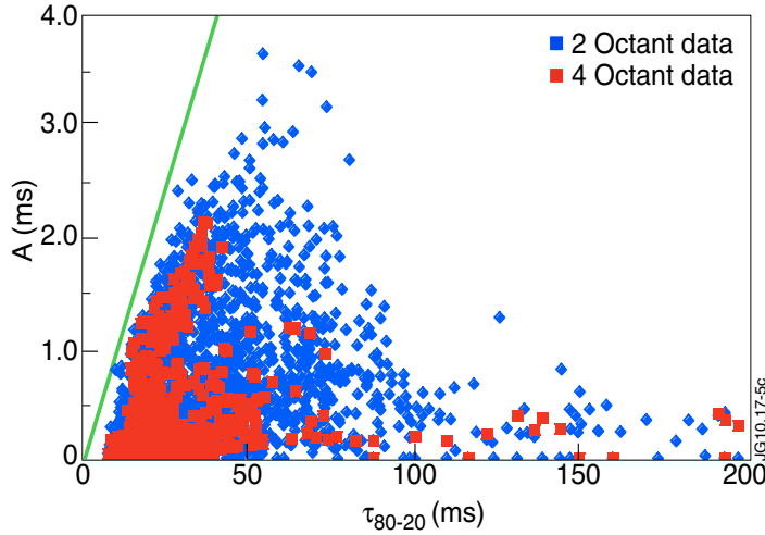
Fig 3 A_{4oct} (red) and \pi/2 A_{2oct} (blue) vs the current quench time extrapolated from time to quench from 80 to 20% of I_p^{dis} (ie. the time from 80 to 20% multiplied by 5/3). The green line is the integral asymmetry if the I_p asymmetry is 10% of I_p for the whole \tau_{80-20} time.
