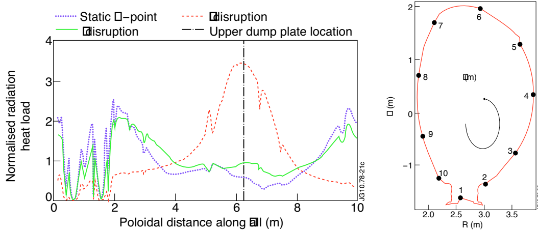
Fig 6 Normalised radiation power load during thermal quench as function of poloidal distance around the wall (as defined in the right figure) for disruptions caused by a density limit, neo-classical tearing mode (NTM) and a VDE. The power loads are normalised by their average values [10].
