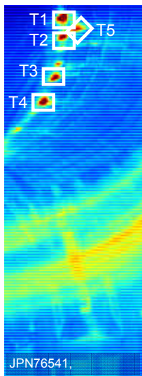
Fig 7 IR view showing 5 tiles being heated strongly during the phase in which the RE current is lost.
