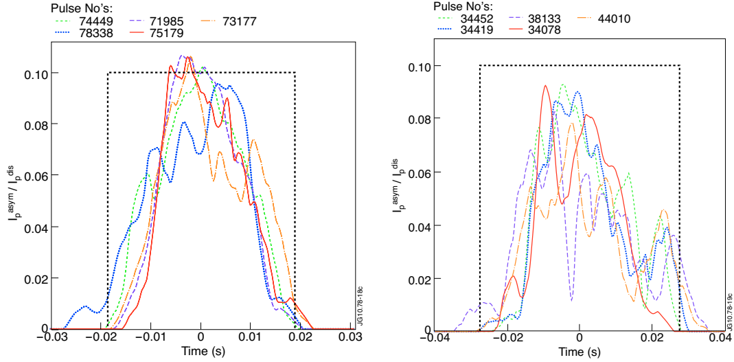
Fig 2 I_p^{asym} / I_p^{dis} for pulses with the maximum A_{4oct} values (left hand figure) and maximum A_{2oct} values (right hand figure). The data are smoothed with a \pm 2 ms rectangular window.
