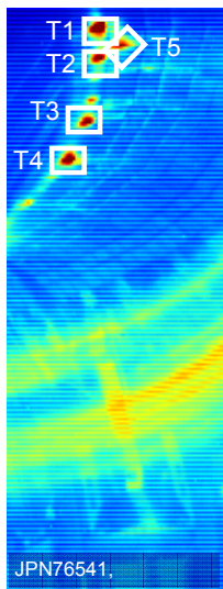
Fig 7 IR view showing 5 tiles being heating strongly during the phase in which the RE current is lost.
