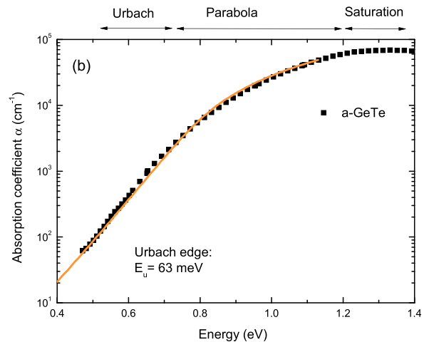
FIG. 4. (a) a-GeTe DOS made of two band tails which fix the Fermi level, indicated by a vertical line, at 0.25 eV above E_v . (b) A fit (full line) of the experimental variations (symbols) of the absorption coefficient measured by PDS.
