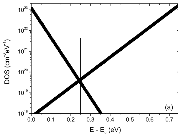
FIG. 4. (a) a-GeTe DOS made of two band tails which fix the Fermi level, indicated by a vertical line, at 0.25 eV above E_v . (b) A fit (full line) of the experimental variations (symbols) of the absorption coefficient measured by PDS.
