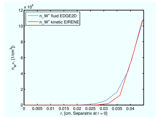
Figure 1: Density profile calculated with fluid and kinetic approach of W^+ at Outer Midplane
