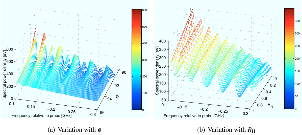
Figure 1: Theoretical spectra calculated with parameters relevant for TEXTOR: n_e = 3 \times 10^{19} \text{ m}^{-3} , T_e = 1.1 \text{ keV} , T_i = 1.1 \text{ keV} , B_t = 2.6 \text{ T} . The spectrum is shown for frequencies from 300 MHz to 100 MHz below the probe frequency corresponding to the range monitored with the modified CTS receiver. In (a) R_H=0.5 while \phi is varied from 91^\circ to 95^\circ . In (b) \phi = 93^\circ while R_H is varied from 0.01 to 0.99.
