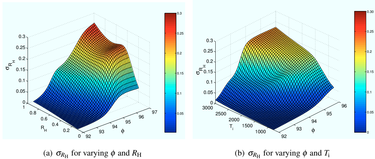
Figure 2: Theoretically calculated posterior uncertainties for model parameters as in Fig. 1 and prior uncertainties: \sigma_{n_e} = 3 \times 10^{18} \text{ m}^{-3} , \sigma_{T_e} = 0.4 \text{ keV} , \sigma_{T_i} = 0.4 \text{ keV} , \sigma_{B_t} = 0.1 \text{ T} , \sigma_{\phi} = 3^\circ , \sigma_{R_H} = 0.5 . In (a) R_H and \phi are varied while other parameters are kept constant. In (b) R_H = 0.5 and \phi and T_i are varied while other parameters are kept constant. \sigma_{R_H} is significantly reduced from its prior value when \phi is close to 90^\circ .
