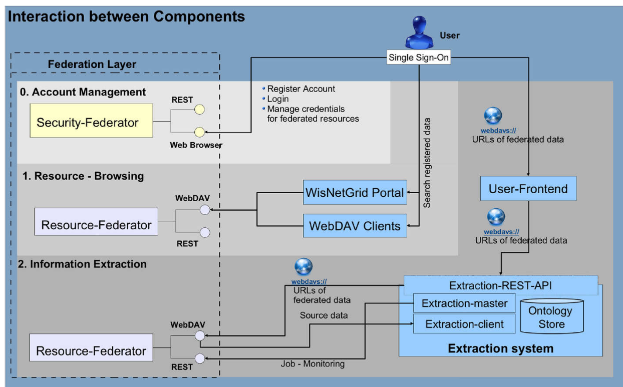
Figure 6 Interface interaction of the extraction system with the resource and security federation layer.
