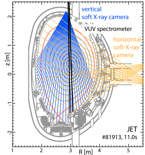
FIG. 1: Diagnostic setup for determining the W-concentration and its poloidal asymmetry. The sight lines of soft X-ray cameras (blue and orange) and of a spectrometer (black) are featured together with the magnetic equilibrium of #81913 at 11.0 s.
