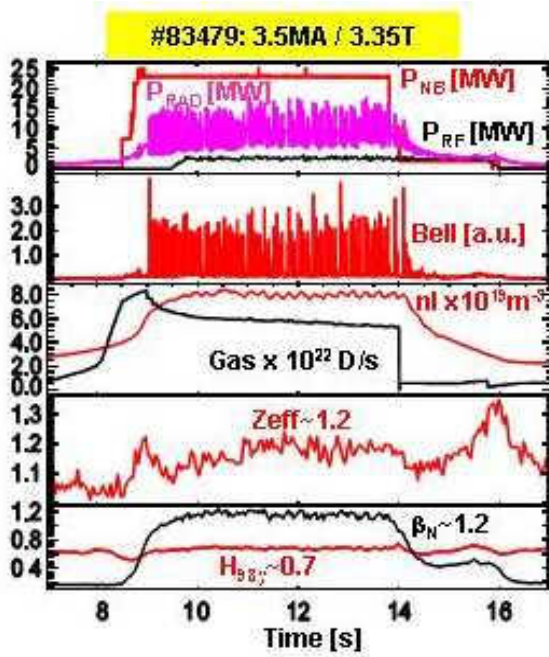
Fig 5: 3.5MA pulse run at JET with the ILW. Note the strong D gas puffing rate and the plasma termination using a tail of ICRH and NBI power for 2s.
