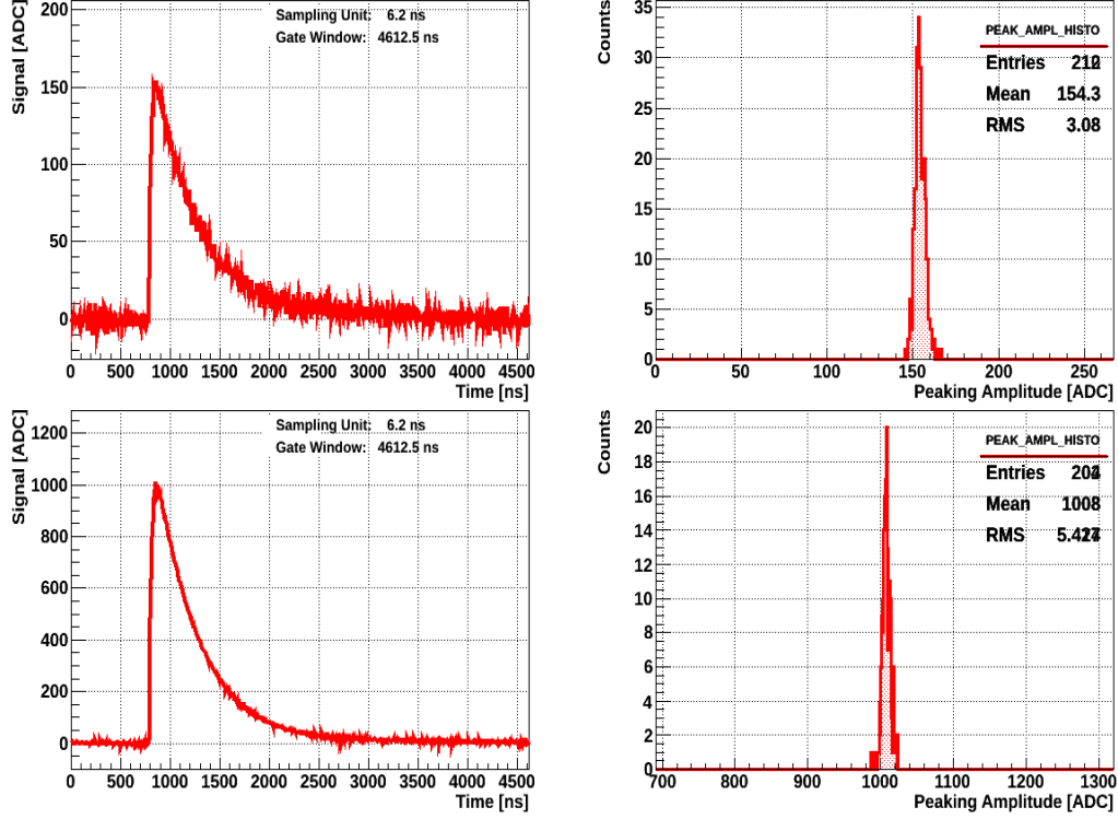
Figure 27: Waveform analysis with the WASA electronics using the developed transimpedance amplifier above described. Measurement done without frequency filtering . Examples obtained with 3 mV (upper panels) and 20 mV (bottom panels) of voltage amplitude provided by the pulse generator.
