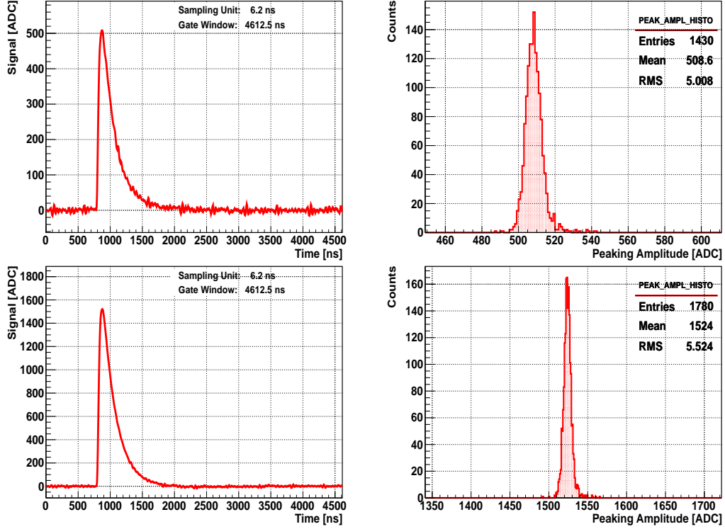
Figure 37: Waveform analysis with the WASA electronics using the developed transimpedance amplifier above described. Measurements done with differential output . These examples were obtained with 5 mV (upper panels) and 15 mV (bottom panels) of voltage amplitude provided by the pulse generator.
