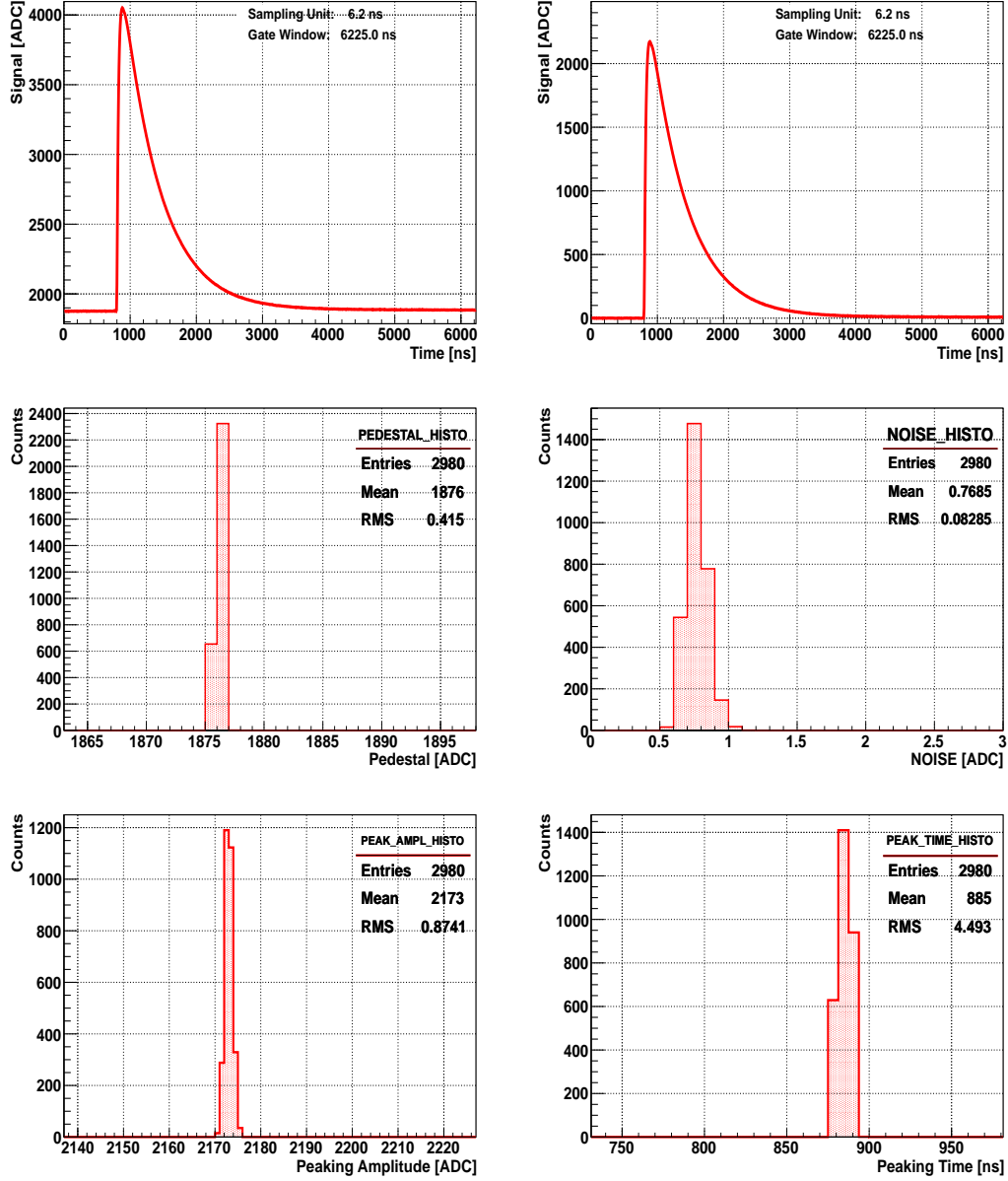
Figure 3: Typical histograms obtained during the waveform analysis with the WASA electronics. These examples were obtained with 1900 mV voltage amplitude provided by the pulse generator.
