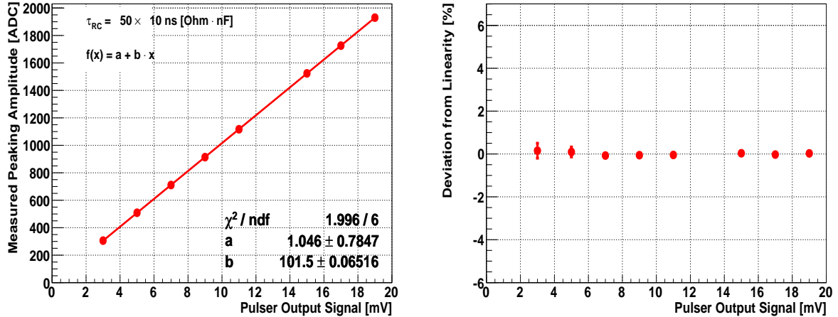
Figure 38: The linearity of the experimental system is here extracted via a linear fit to the data of the scan w.r.t. the amplitude of the input signal sent by the pulser to the WASA board (left panel). The deviation to linearity shows that the system is linear within 1% through all available ADC range (right panel). This measurement was performed with the new transimpedance amplifier and with differential output .
