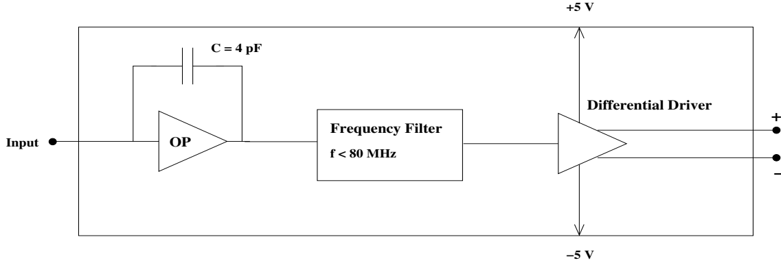
Figure 26: Schematic of the developed amplifier made of, in sequence, the transimpedance in parallel with a very low capacitance, a frequency filter and a differential driver.
