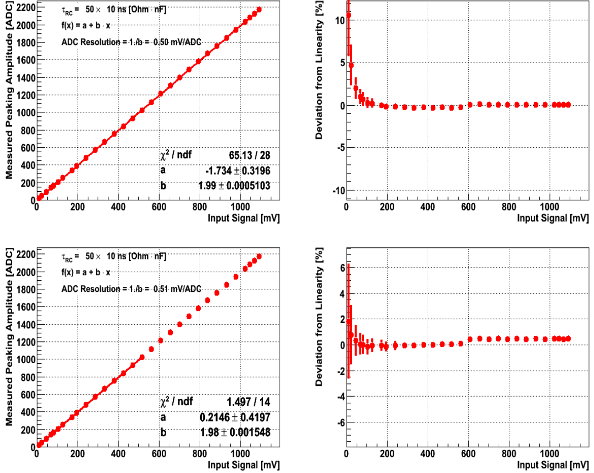
Figure 4: The ADC resolution is here extracted via a linear fit to the data of the scan w.r.t. the amplitude of the input voltage pulse.
