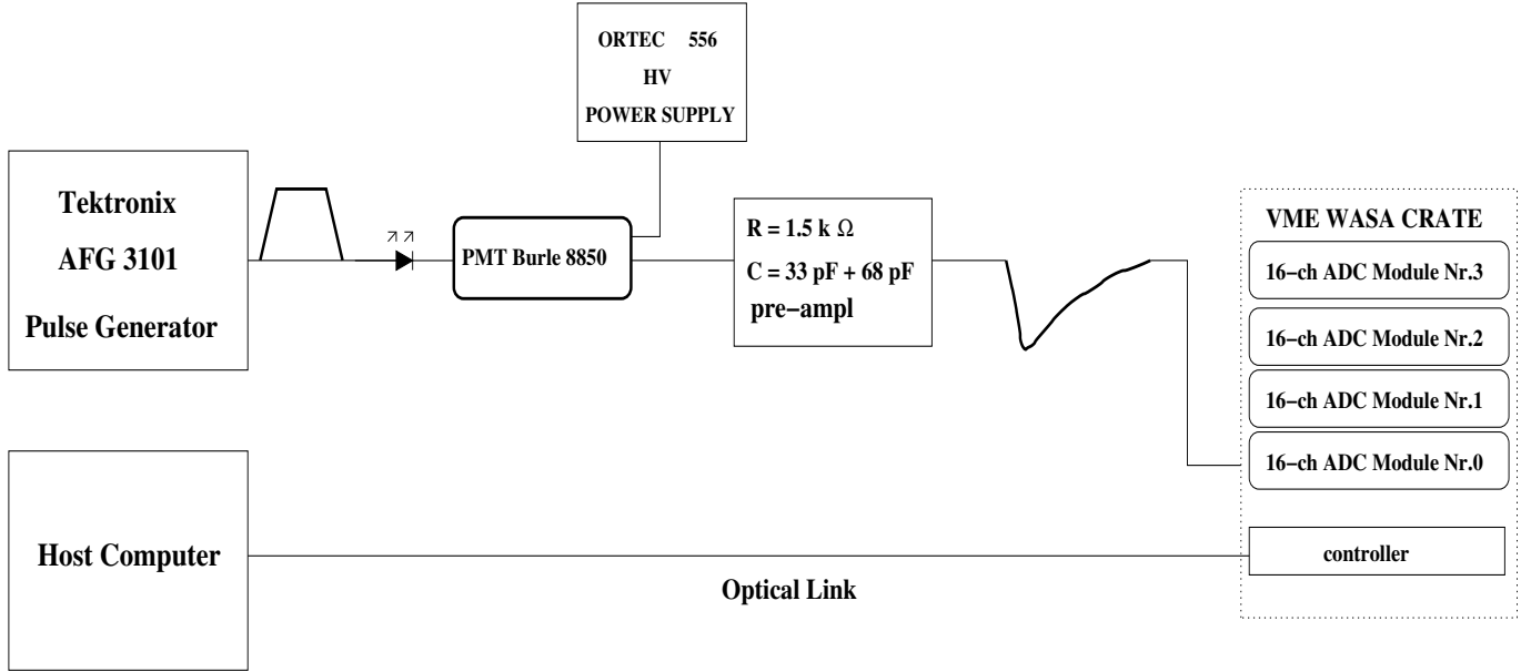
Figure 8: Test-bench setup used for the waveform analysis with the WASA readout system at FZJ using the signal generated by a photomultiplier. A similar experimental setup is used when using the ACQIRIS system: here network twisted cables are used for transmitting the data to the host computer.
