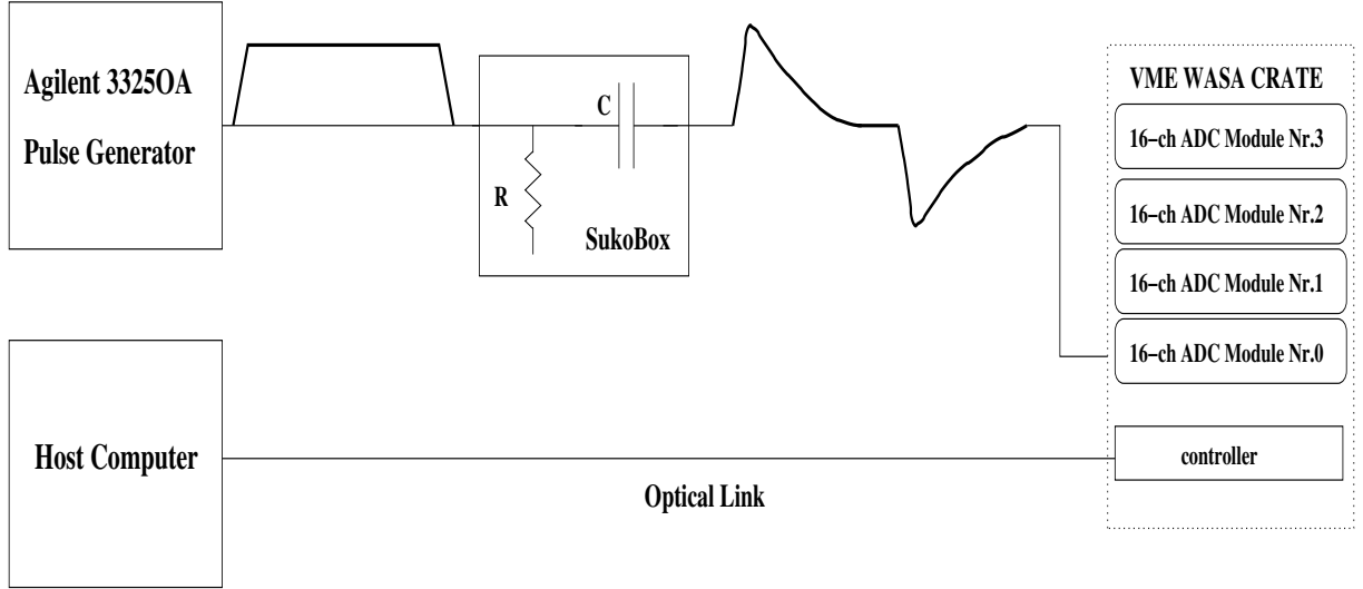
Figure 2: Test-bench setup used for the waveform analysis with the WASA readout system at FZJ. A similar experimental setup is used when using the ACQIRIS system: here network twisted cables are used for transmitting the data to the host computer.
