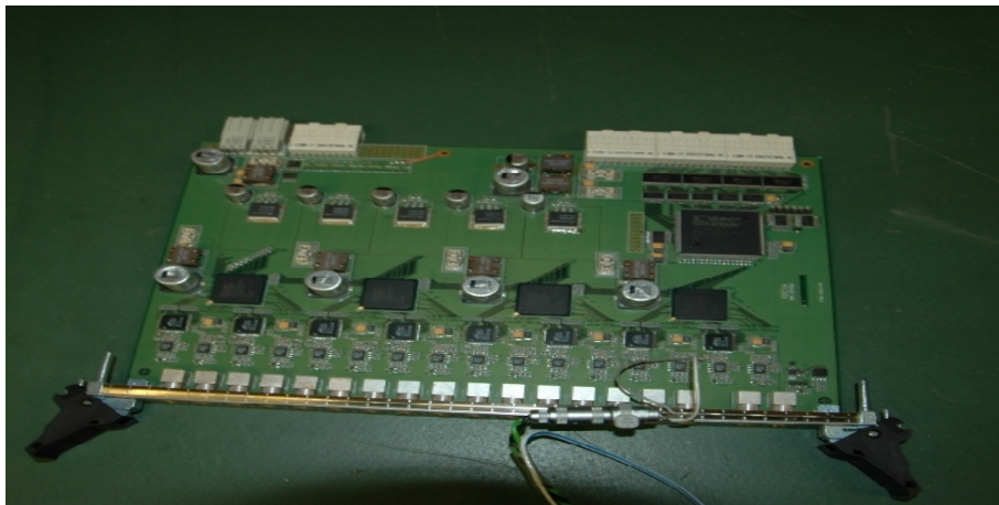
Figure 1: QDC module of the WASA electronics with the sixteen 50 Ohm Lemo connectors for the input signals. Visible at the front-end side is the ad-hoc made connection to the ADC to test the processing of differential signals.
