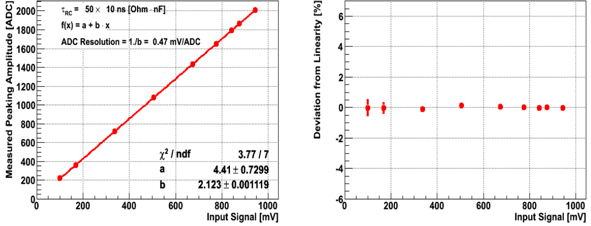
Figure 33: The ADC resolution is here extracted via a linear fit to the data of the linear scan in the amplitude of the input signal to the WASA board (left panel). The deviation to linearity shows a system linear within 1% within all available ADC range (right panel). The measurement was performed with the new transimpedance amplifier and with frequency filtering .
