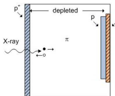
Fig. 8: Sketch of the avalanche photodiode operation principle. The incident radiation interacts in the \pi -region that constitutes most of the diode thickness. The electric field at the \text{pn}^+ region is very high, so that charge multiplication occurs.
