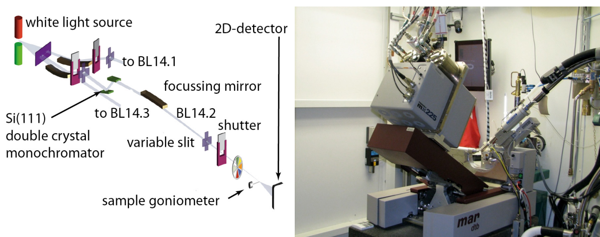
Fig. 8: Schematic view of the beamline 14.2 of BESSY beginning with the magnet structure which is used as a white light X-ray photon source. On the right a picture taken from the experimental hutch of beamline 14.1 is shown. The beam enters from the right and the sample goniometer is mounted horizontally from the left. A cryostream sample environment to stabilize the sample temperature is discernible pointing towards the sample from the top right corner. Pictures kindly provided by Dr. Uwe Müller, BESSY.
