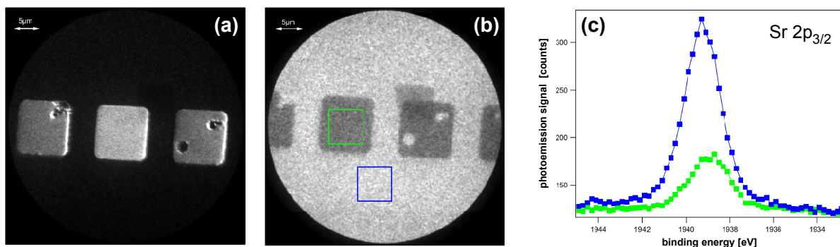
Figure 29: Laterally resolved HAXPES on Au microstructures on SrTiO 3 . (a) threshold photoemission, (b) Sr 2p 3/2 photoelectron distribution at h\nu = 6500 eV, and (c) local photoelectron spectra from the regions of interest (blue, green).
