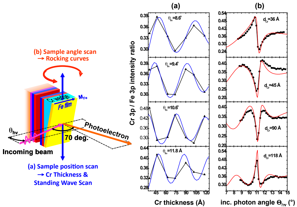
Figure 31: Experimental and calculated Cr3p/Fe3p ratios for two types of standing wave scan for the sample shown in Figure 21: (a) Scanning the sample along x at fixed incidence angle, as indicated in Figure 30, and (b) scanning the sample polar angle with fixed x position (or Cr thickness). The best-fit theory curves are for the parameters shown at the left of Figure 24(a). From ref. [66].
