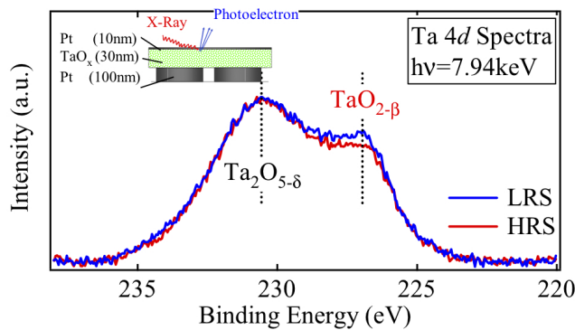
Figure 27: Hard x-ray photoemission spectra from Ta 2 O 5 in the high (HRS) and low resistive state (LRS). From [58].
