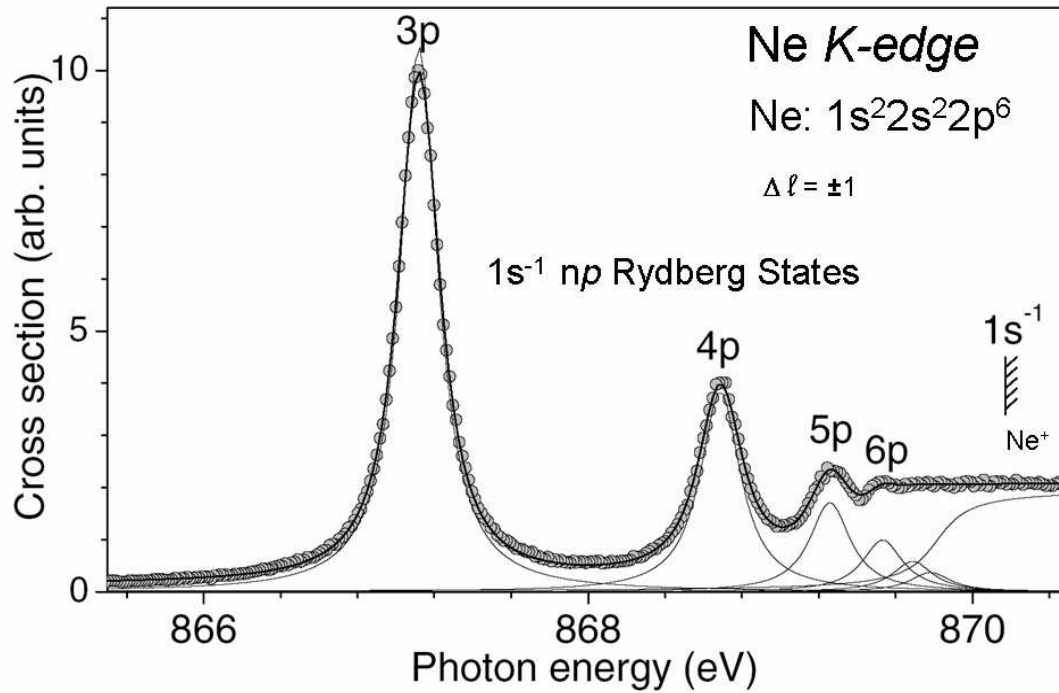
Fig. 7: total cross section for photoionization of Ne in CO 2 at K edge absorption. The curves are fits to the data with a Gaussian with FWHM fixed to 66 meV [31].
