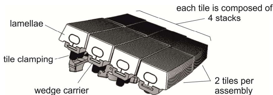
FIG 2 One of the 48 assemblies which compose the solid tungsten row in the divertor (tile 5). The torus axis (high field side) is on the left of the picture.
