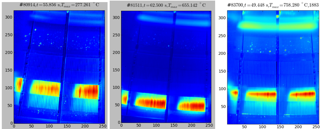
FIG. 4 Top views of the bulk tungsten tile under various conditions (different stacks wetted) with an infrared camera (KL9B [14]).
