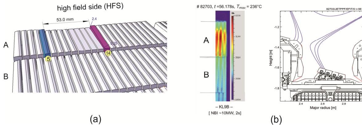
FIG. 5 (a) Arrangement of tungsten lamellae for deliberate melting, and (b) operation with OSP moved to stack A during JET pulse # 82703
