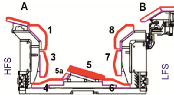
FIG. 1 Cross section of the current JET divertor. Tiles 1 and 3, where the inner strike point (ISP) is placed in the following, are coated with Mo/W layers of 25 \mu\text{m} and 12 \mu\text{m} , respectively. Tile 5 (within the range of the OSP) is made of bulk tungsten.
