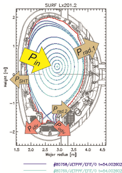
FIG. 3 Power fluxes that were considered in the power balance to the outer divertor leg
