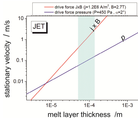
FIG. 6 One of the model predictions for the driving force acting on a melt layer in JET. The shaded region indicates the range of expected thickness. (by courtesy of G. Sergienko)
