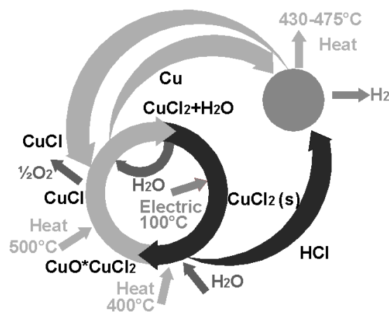
Figure 3: Simplified schematic diagram of Cu-Cl cycle.
